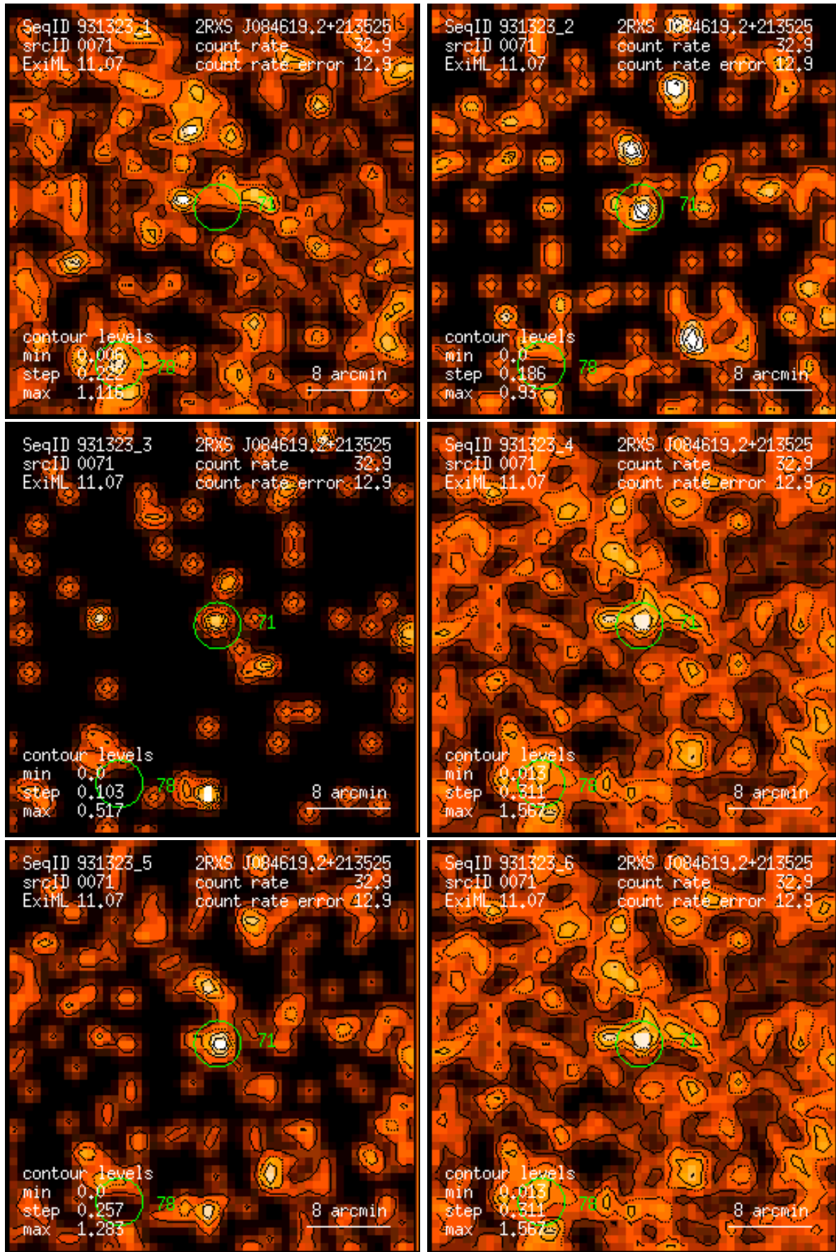
Figure 71: RASS 931323: detection 0071: band rate images, Gaussian filter: (1) PSPC channels 11 – 41, (2) 52 – 90, (3) 91 – 201, (4) 11 – 235, (5) 52 – 201, (6) 11 – 201. Broad band rates in counts/ks. Band rate contour levels in counts/ks/arcmin 2 .
