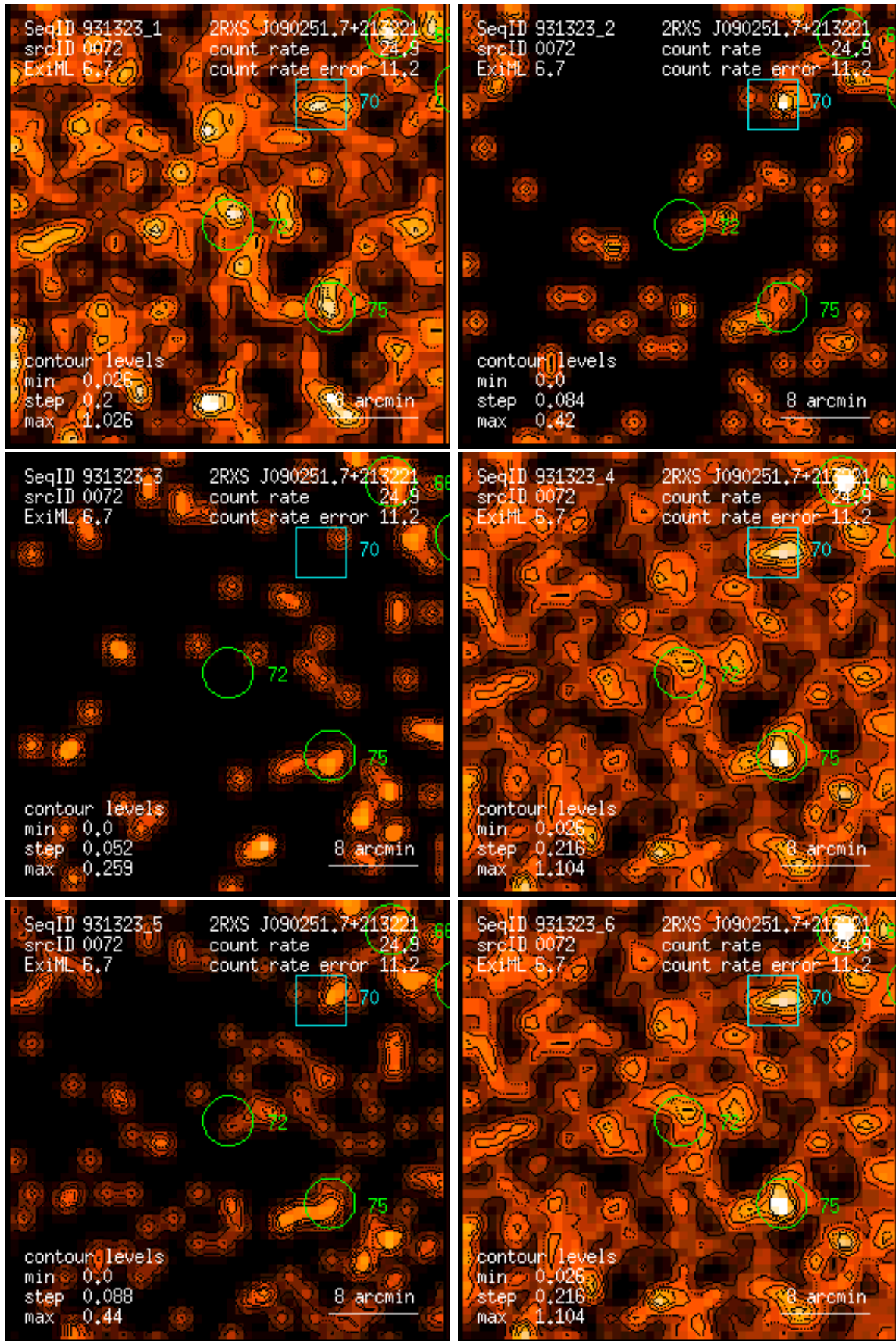
Figure 72: RASS 931323: detection 0072: band rate images, Gaussian filter: (1) PSPC channels 11 – 41, (2) 52 – 90, (3) 91 – 201, (4) 11 – 235, (5) 52 – 201, (6) 11 – 201. Broad band rates in counts/ks. Band rate contour levels in counts/ks/arcmin 2 .
