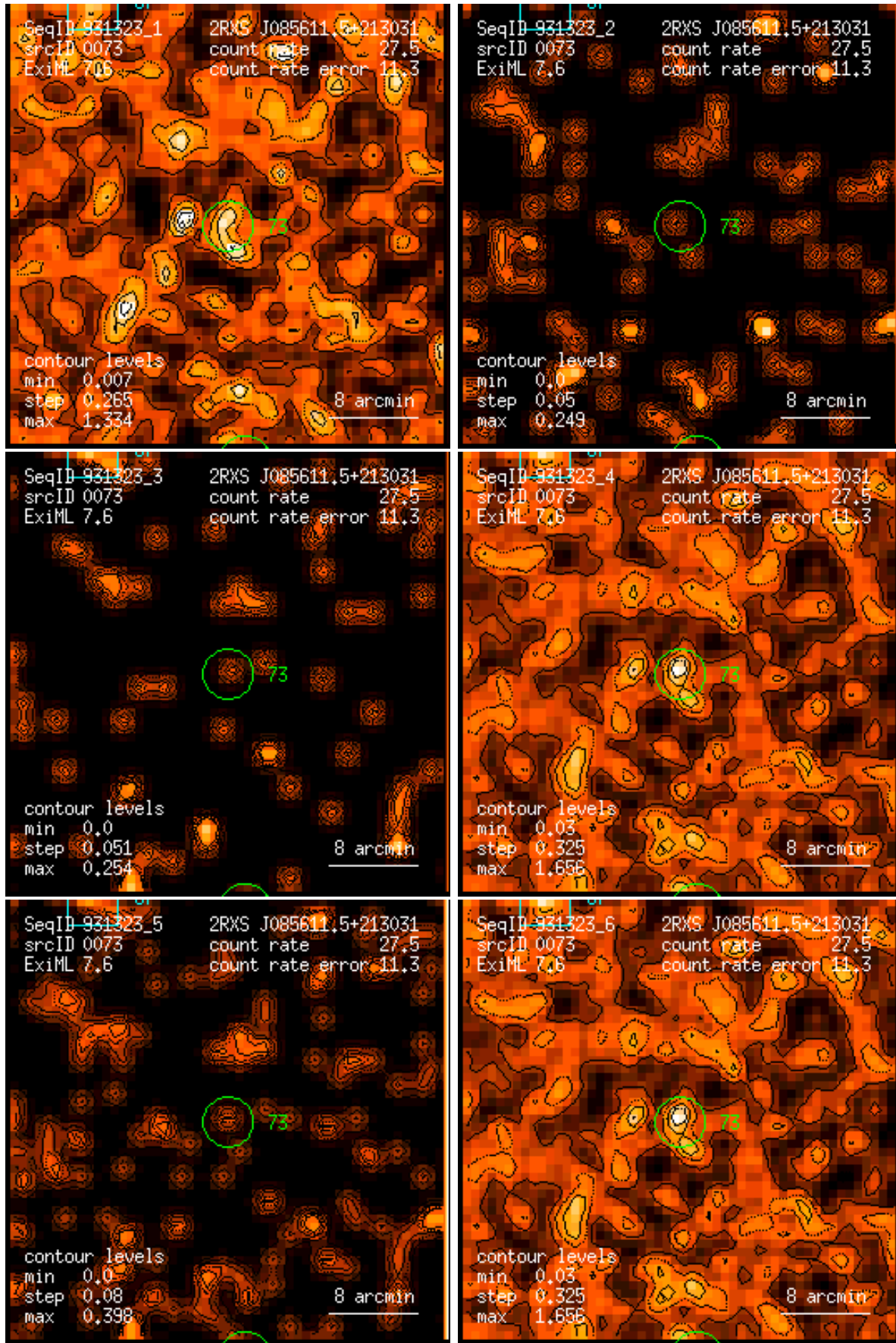
Figure 73: RASS 931323: detection 0073: band rate images, Gaussian filter: (1) PSPC channels 11 – 41, (2) 52 – 90, (3) 91 – 201, (4) 11 – 235, (5) 52 – 201, (6) 11 – 201. Broad band rates in counts/ks. Band rate contour levels in counts/ks/arcmin 2 .
