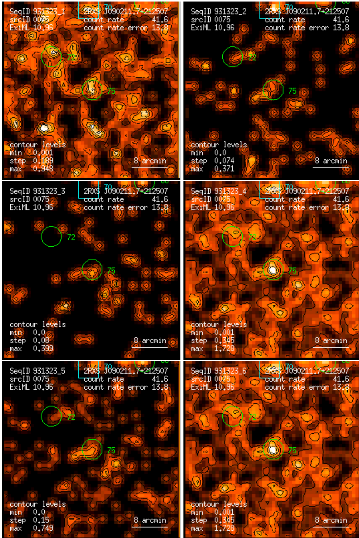
Figure 75: RASS 931323: detection 0075: band rate images, Gaussian filter: (1) PSPC channels 11 – 41, (2) 52 – 90, (3) 91 – 201, (4) 11 – 235, (5) 52 – 201, (6) 11 – 201. Broad band rates in counts/ks. Band rate contour levels in counts/ks/arcmin 2 .
