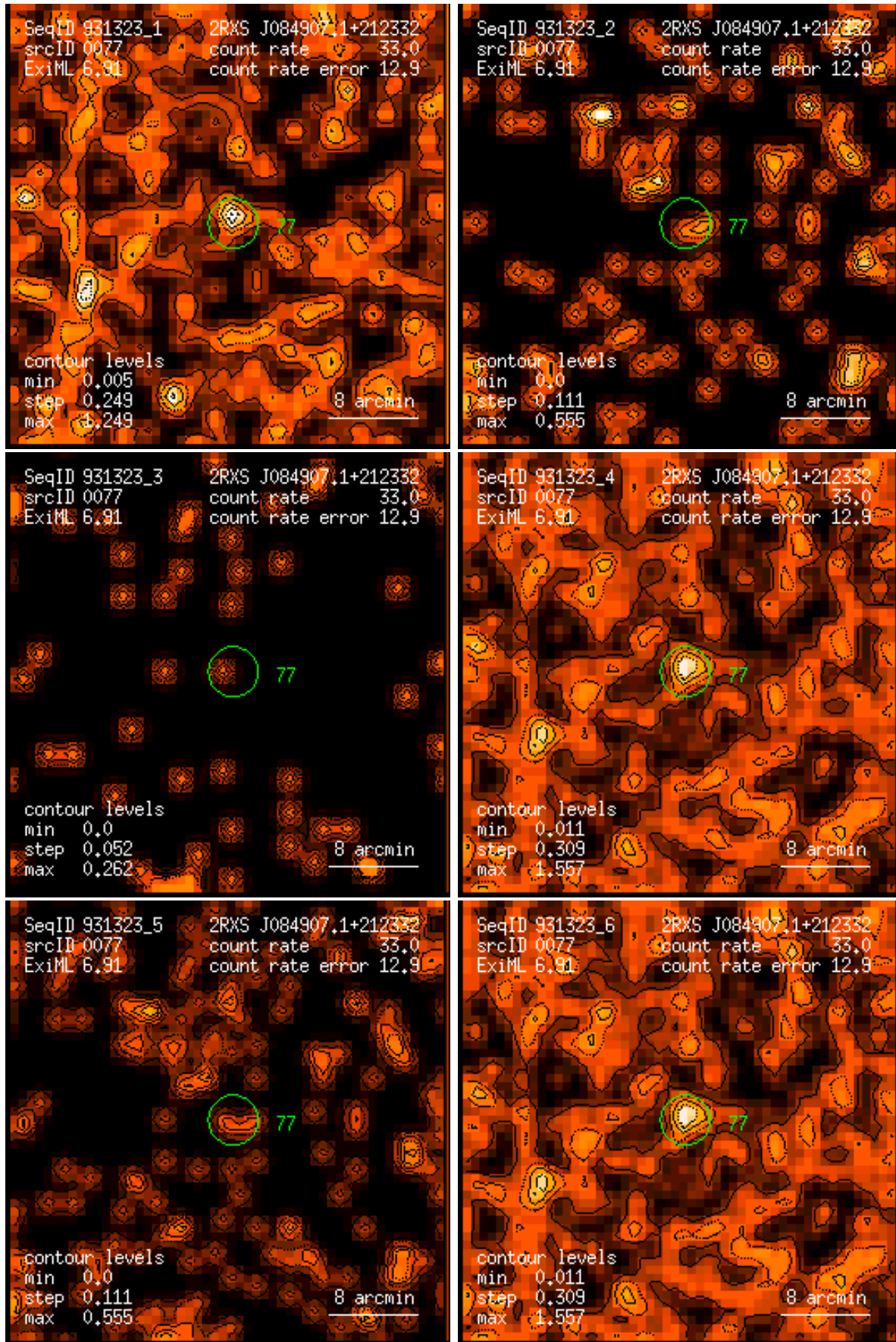
Figure 77: RASS 931323: detection 0077: band rate images, Gaussian filter: (1) PSPC channels 11 – 41, (2) 52 – 90, (3) 91 – 201, (4) 11 – 235, (5) 52 – 201, (6) 11 – 201. Broad band rates in counts/ks. Band rate contour levels in counts/ks/arcmin 2 .
