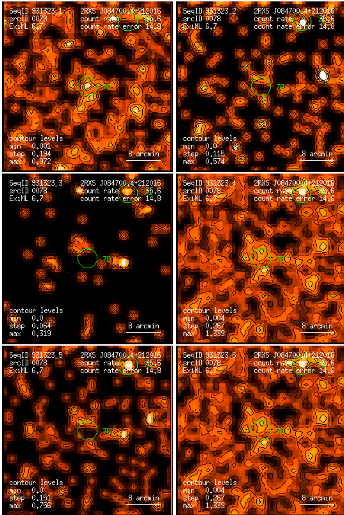
Figure 78: RASS 931323: detection 0078: band rate images, Gaussian filter: (1) PSPC channels 11 – 41, (2) 52 – 90, (3) 91 – 201, (4) 11 – 235, (5) 52 – 201, (6) 11 – 201. Broad band rates in counts/ks. Band rate contour levels in counts/ks/arcmin 2 .
