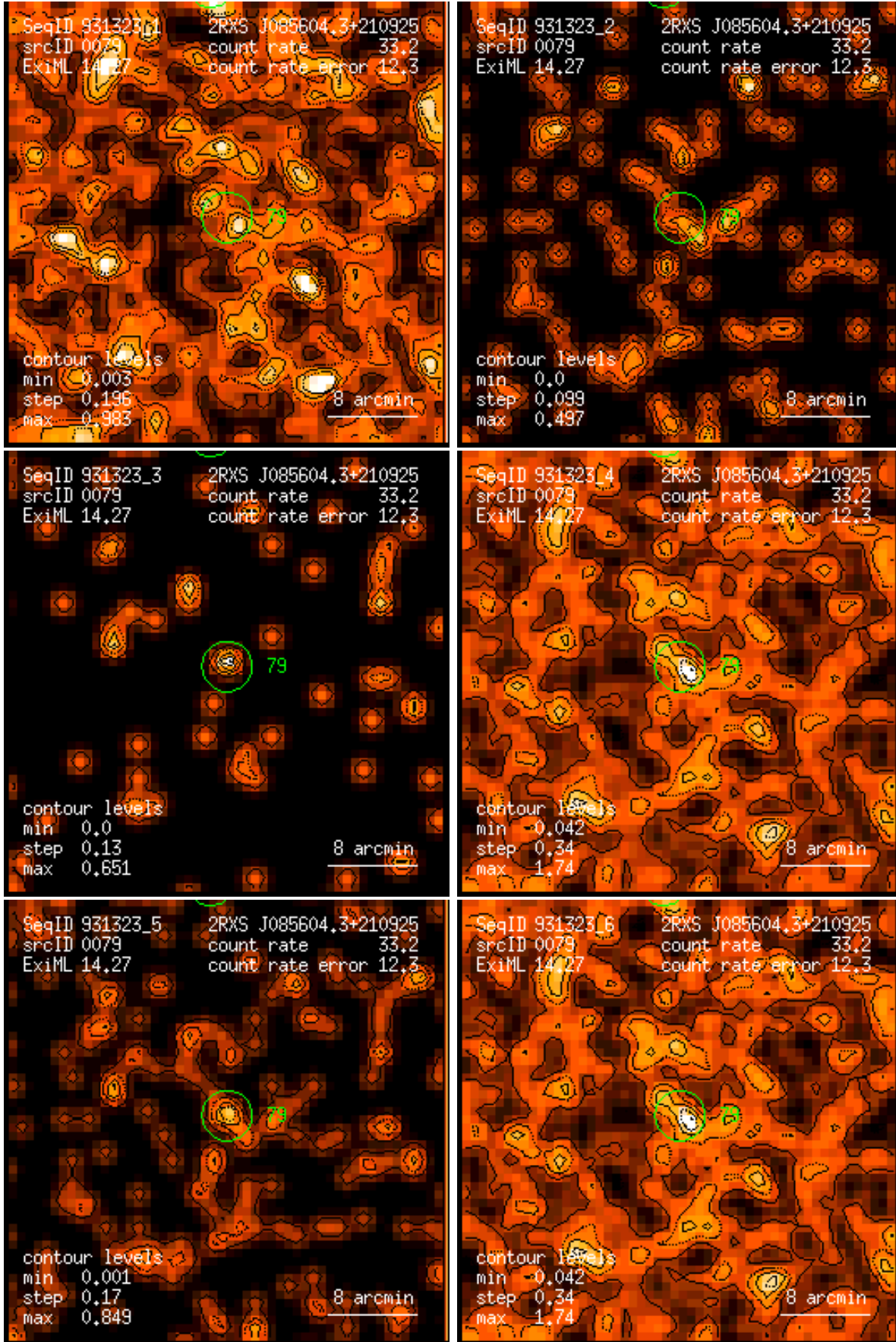
Figure 79: RASS 931323: detection 0079: band rate images, Gaussian filter: (1) PSPC channels 11 – 41, (2) 52 – 90, (3) 91 – 201, (4) 11 – 235, (5) 52 – 201, (6) 11 – 201. Broad band rates in counts/ks. Band rate contour levels in counts/ks/arcmin 2 .
