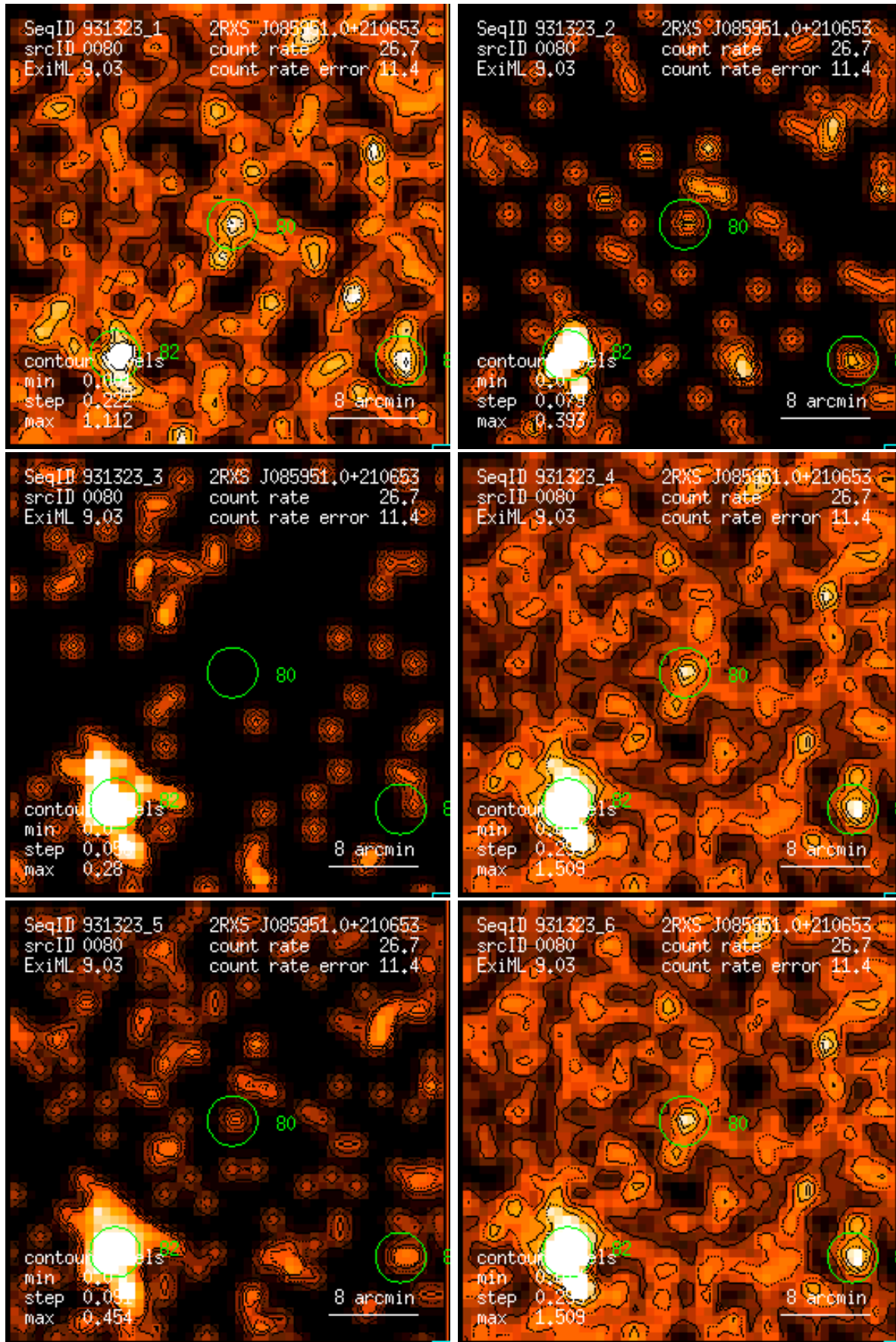
Figure 80: RASS 931323: detection 0080: band rate images, Gaussian filter: (1) PSPC channels 11 – 41, (2) 52 – 90, (3) 91 – 201, (4) 11 – 235, (5) 52 – 201, (6) 11 – 201. Broad band rates in counts/ks. Band rate contour levels in counts/ks/arcmin 2 .
