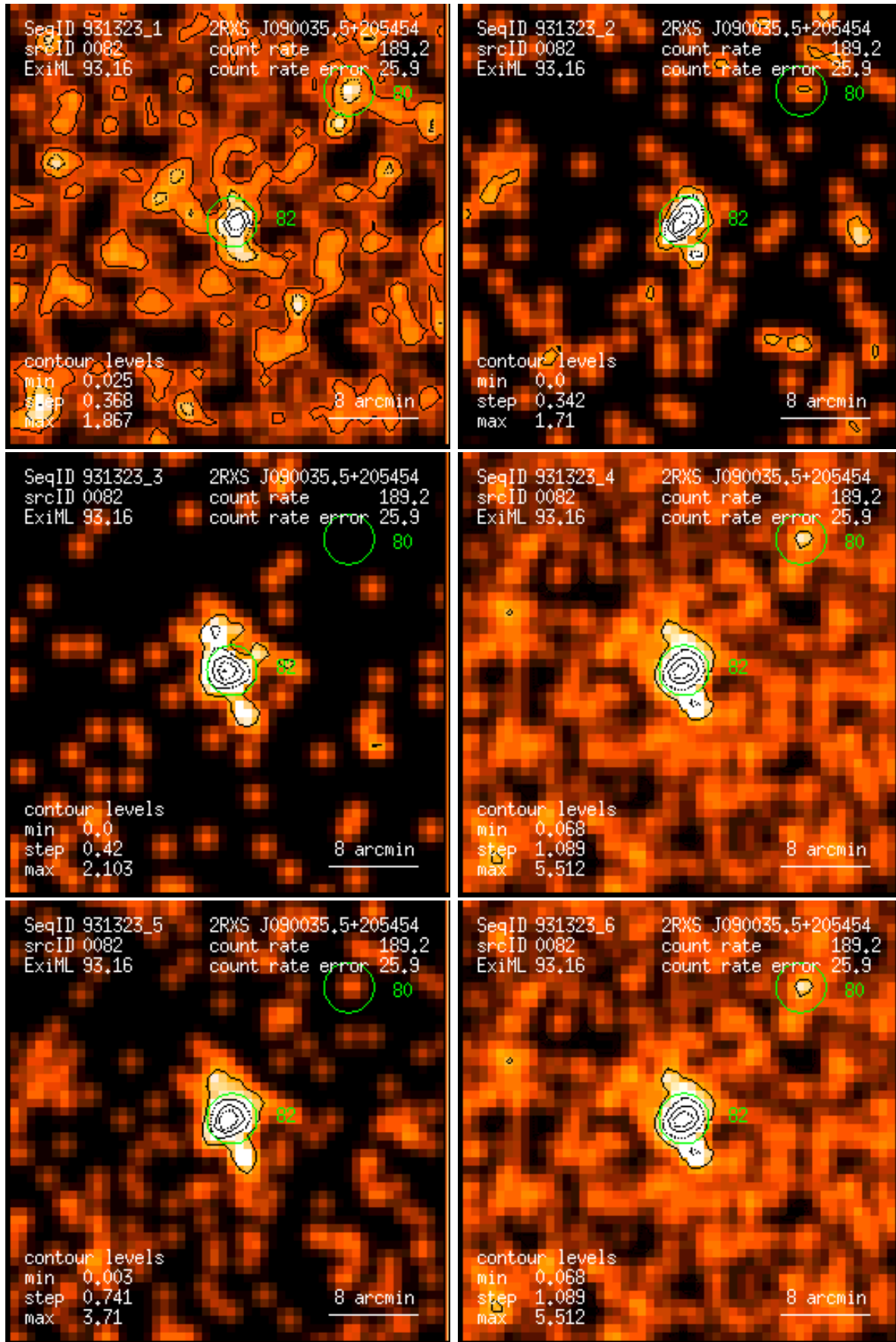
Figure 82: RASS 931323: detection 0082: band rate images, Gaussian filter: (1) PSPC channels 11 – 41, (2) 52 – 90, (3) 91 – 201, (4) 11 – 235, (5) 52 – 201, (6) 11 – 201. Broad band rates in counts/ks. Band rate contour levels in counts/ks/arcmin 2 .
