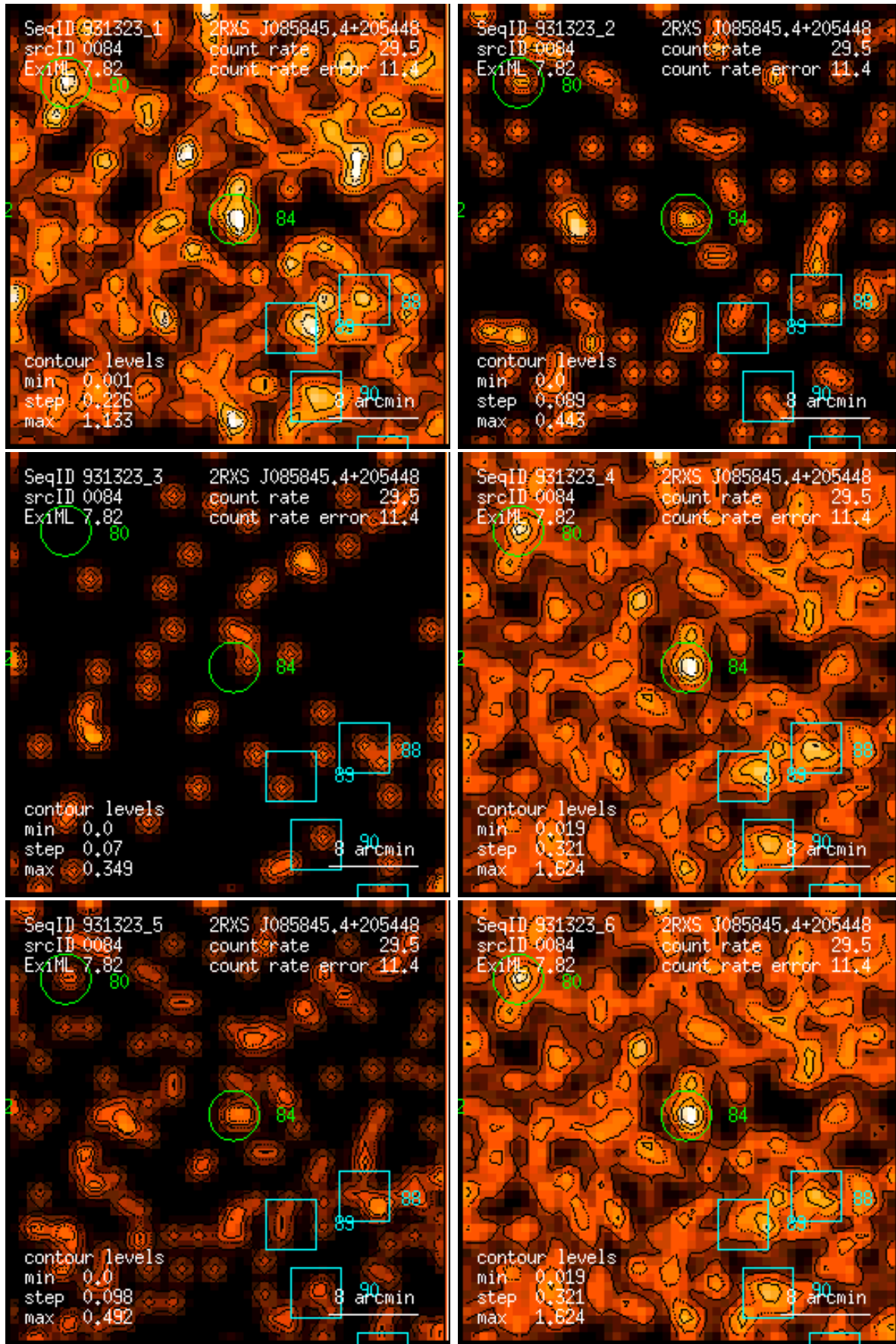
Figure 84: RASS 931323: detection 0084: band rate images, Gaussian filter: (1) PSPC channels 11 – 41, (2) 52 – 90, (3) 91 – 201, (4) 11 – 235, (5) 52 – 201, (6) 11 – 201. Broad band rates in counts/ks. Band rate contour levels in counts/ks/arcmin 2 .
