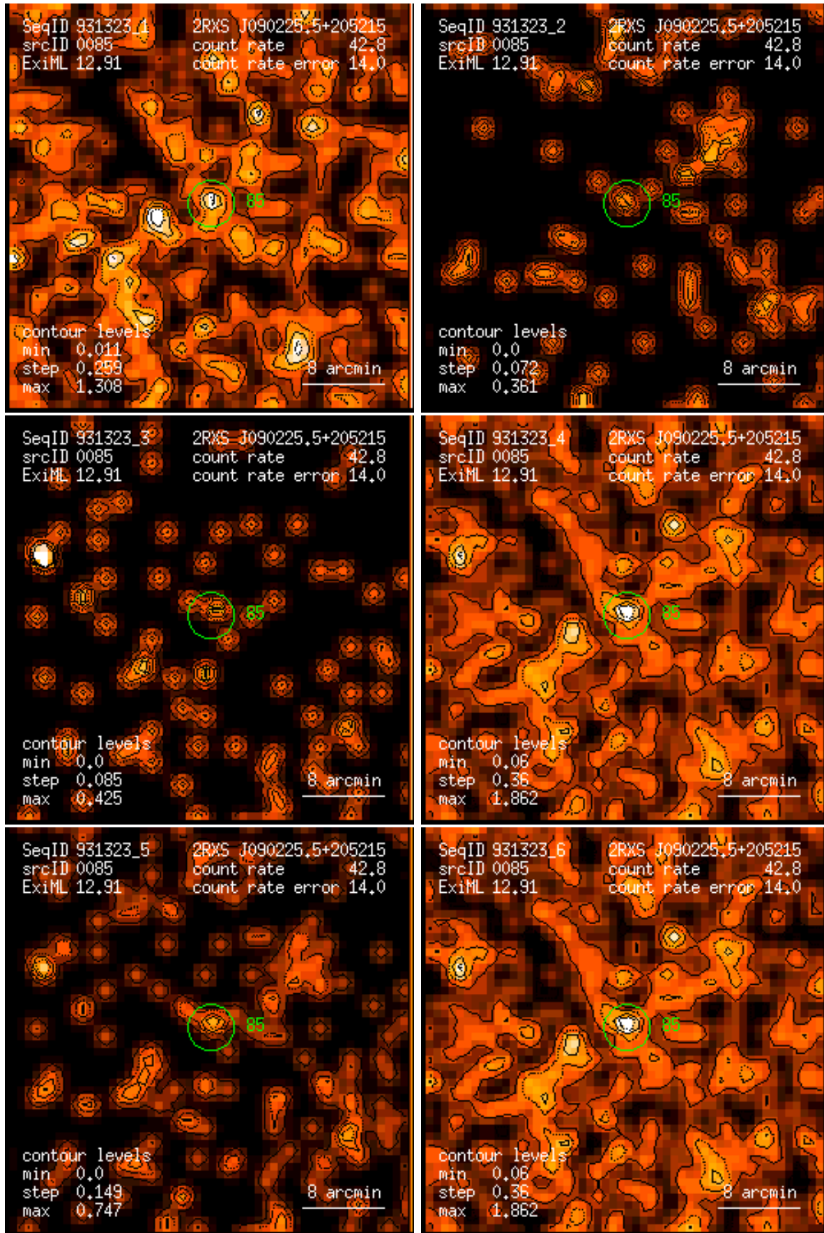
Figure 85: RASS 931323: detection 0085: band rate images, Gaussian filter: (1) PSPC channels 11 – 41, (2) 52 – 90, (3) 91 – 201, (4) 11 – 235, (5) 52 – 201, (6) 11 – 201. Broad band rates in counts/ks. Band rate contour levels in counts/ks/arcmin 2 .
