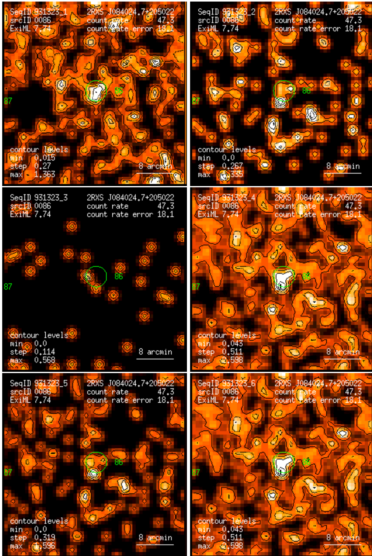
Figure 86: RASS 931323: detection 0086: band rate images, Gaussian filter: (1) PSPC channels 11 – 41, (2) 52 – 90, (3) 91 – 201, (4) 11 – 235, (5) 52 – 201, (6) 11 – 201. Broad band rates in counts/ks. Band rate contour levels in counts/ks/arcmin 2 .
