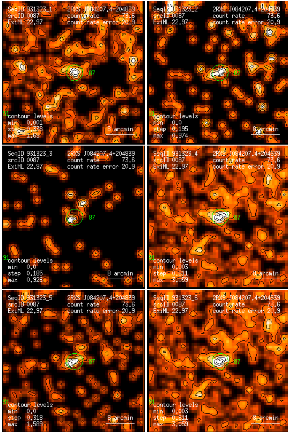
Figure 87: RASS 931323: detection 0087: band rate images, Gaussian filter: (1) PSPC channels 11 – 41, (2) 52 – 90, (3) 91 – 201, (4) 11 – 235, (5) 52 – 201, (6) 11 – 201. Broad band rates in counts/ks. Band rate contour levels in counts/ks/arcmin 2 .
