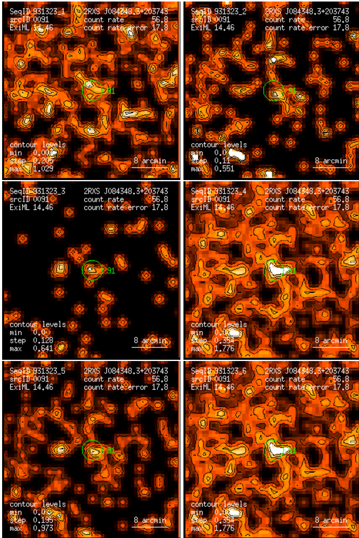
Figure 91: RASS 931323: detection 0091: band rate images, Gaussian filter: (1) PSPC channels 11 – 41, (2) 52 – 90, (3) 91 – 201, (4) 11 – 235, (5) 52 – 201, (6) 11 – 201. Broad band rates in counts/ks. Band rate contour levels in counts/ks/arcmin 2 .
