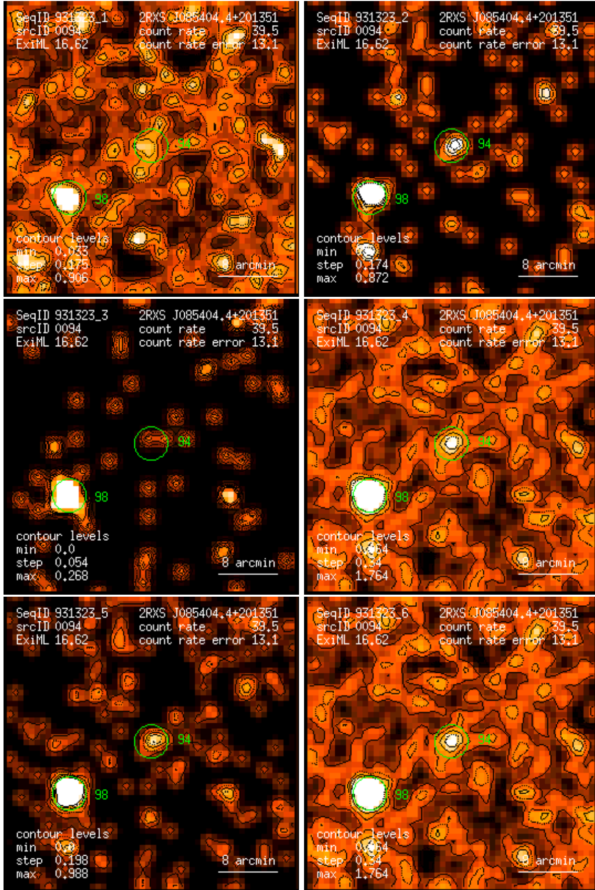
Figure 94: RASS 931323: detection 0094: band rate images, Gaussian filter: (1) PSPC channels 11 – 41, (2) 52 – 90, (3) 91 – 201, (4) 11 – 235, (5) 52 – 201, (6) 11 – 201. Broad band rates in counts/ks. Band rate contour levels in counts/ks/arcmin 2 .
