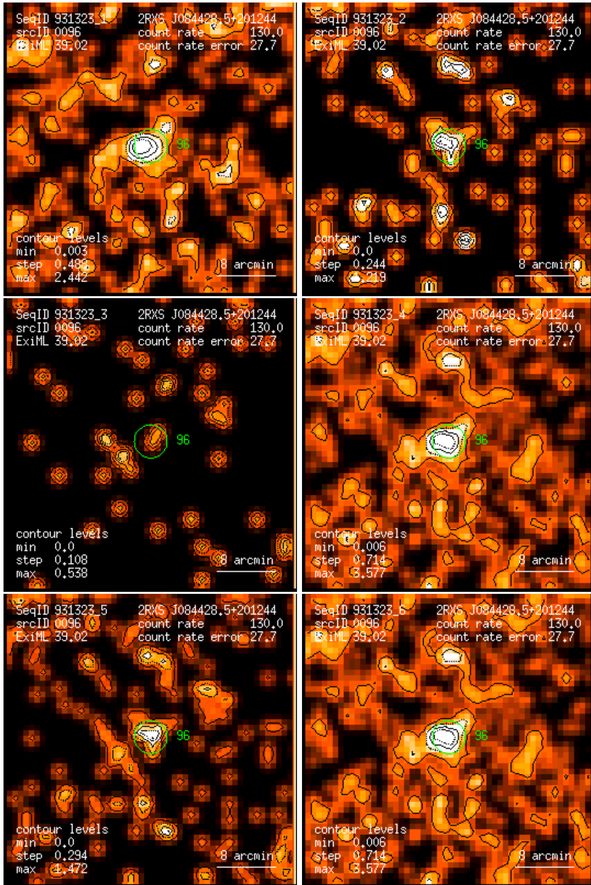
Figure 96: RASS 931323: detection 0096: band rate images, Gaussian filter: (1) PSPC channels 11 – 41, (2) 52 – 90, (3) 91 – 201, (4) 11 – 235, (5) 52 – 201, (6) 11 – 201. Broad band rates in counts/ks. Band rate contour levels in counts/ks/arcmin 2 .
