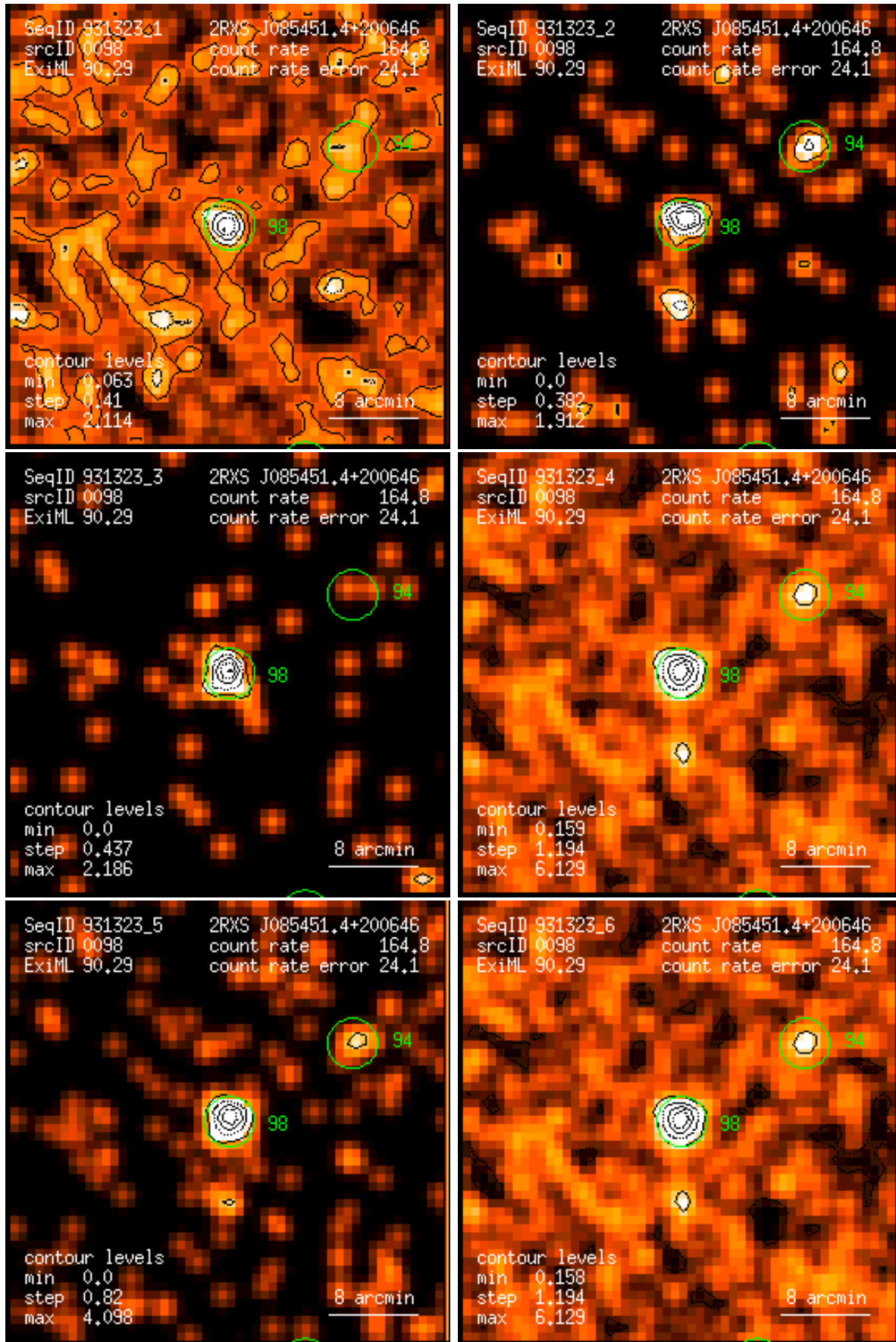
Figure 98: RASS 931323: detection 0098: band rate images, Gaussian filter: (1) PSPC channels 11 – 41, (2) 52 – 90, (3) 91 – 201, (4) 11 – 235, (5) 52 – 201, (6) 11 – 201. Broad band rates in counts/ks. Band rate contour levels in counts/ks/arcmin 2 .
