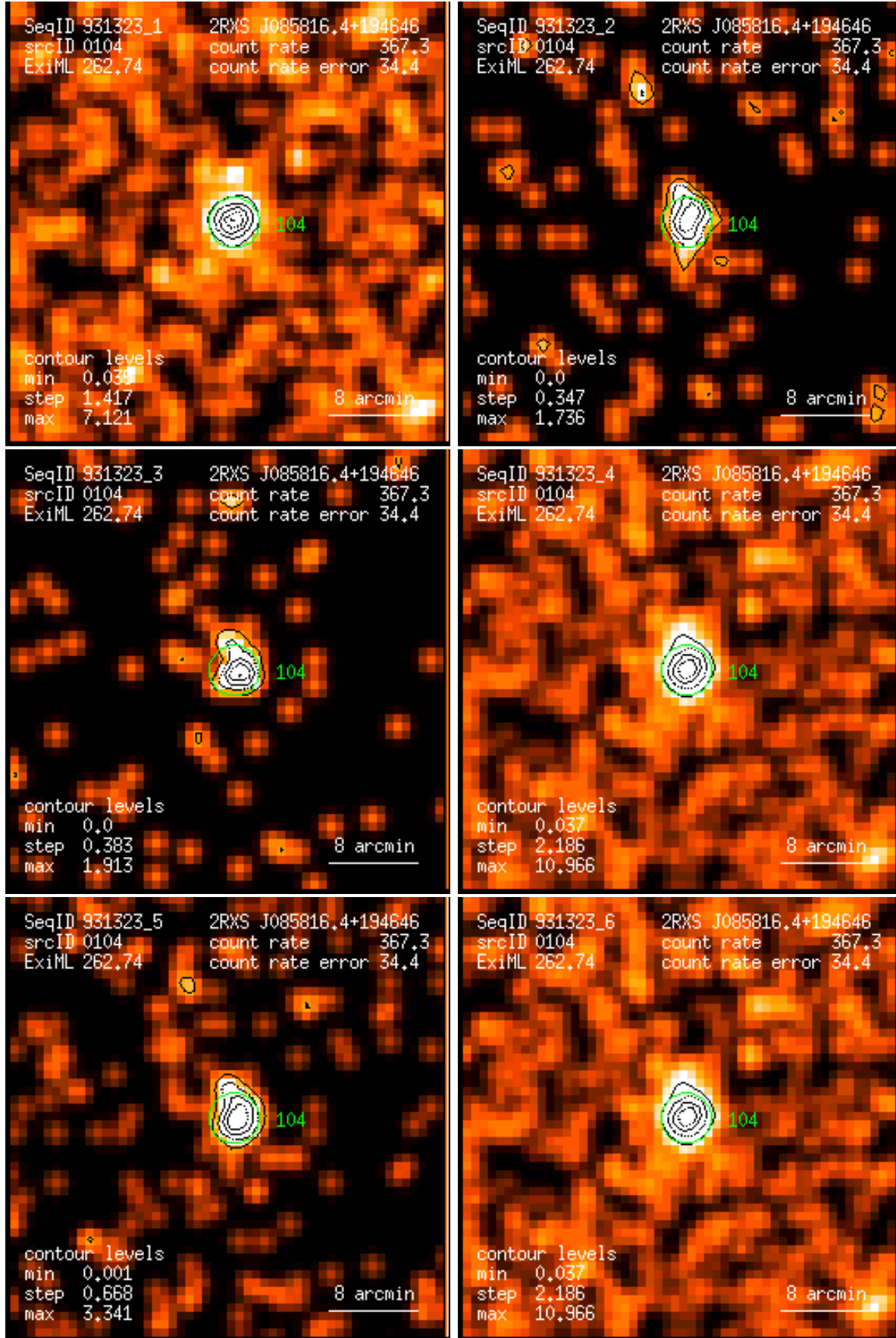
Figure 104: RASS 931323: detection 0104: band rate images, Gaussian filter: (1) PSPC channels 11 – 41, (2) 52 – 90, (3) 91 – 201, (4) 11 – 235, (5) 52 – 201, (6) 11 – 201. Broad band rates in counts/ks. Band rate contour levels in counts/ks/arcmin 2 .
