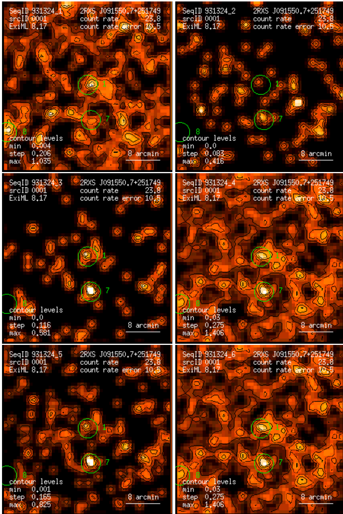
Figure 1: RASS 931324: detection 0001: band rate images, Gaussian filter: (1) PSPC channels 11 – 41, (2) 52 – 90, (3) 91 – 201, (4) 11 – 235, (5) 52 – 201, (6) 11 – 201. Broad band rates in counts/ks. Band rate contour levels in counts/ks/arcmin 2 .
