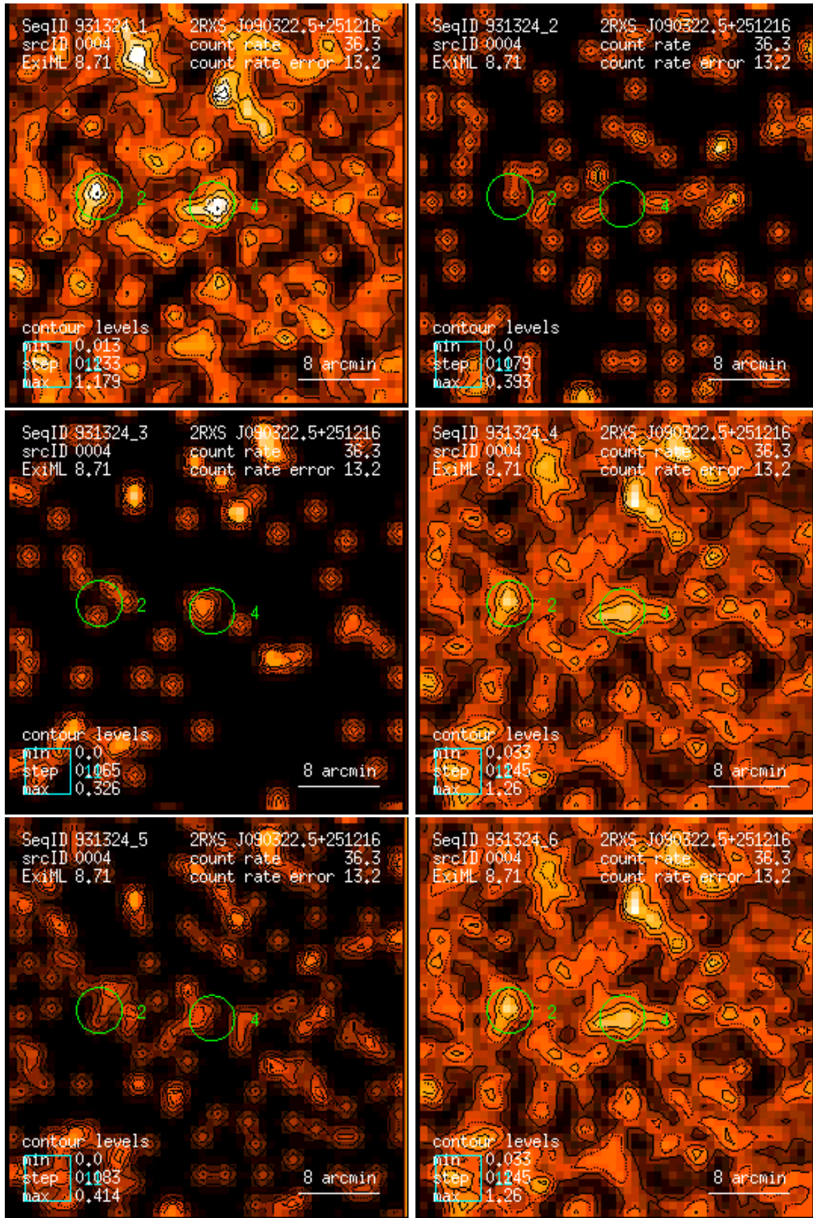
Figure 4: RASS 931324: detection 0004: band rate images, Gaussian filter: (1) PSPC channels 11 – 41, (2) 52 – 90, (3) 91 – 201, (4) 11 – 235, (5) 52 – 201, (6) 11 – 201. Broad band rates in counts/ks. Band rate contour levels in counts/ks/arcmin 2 .
