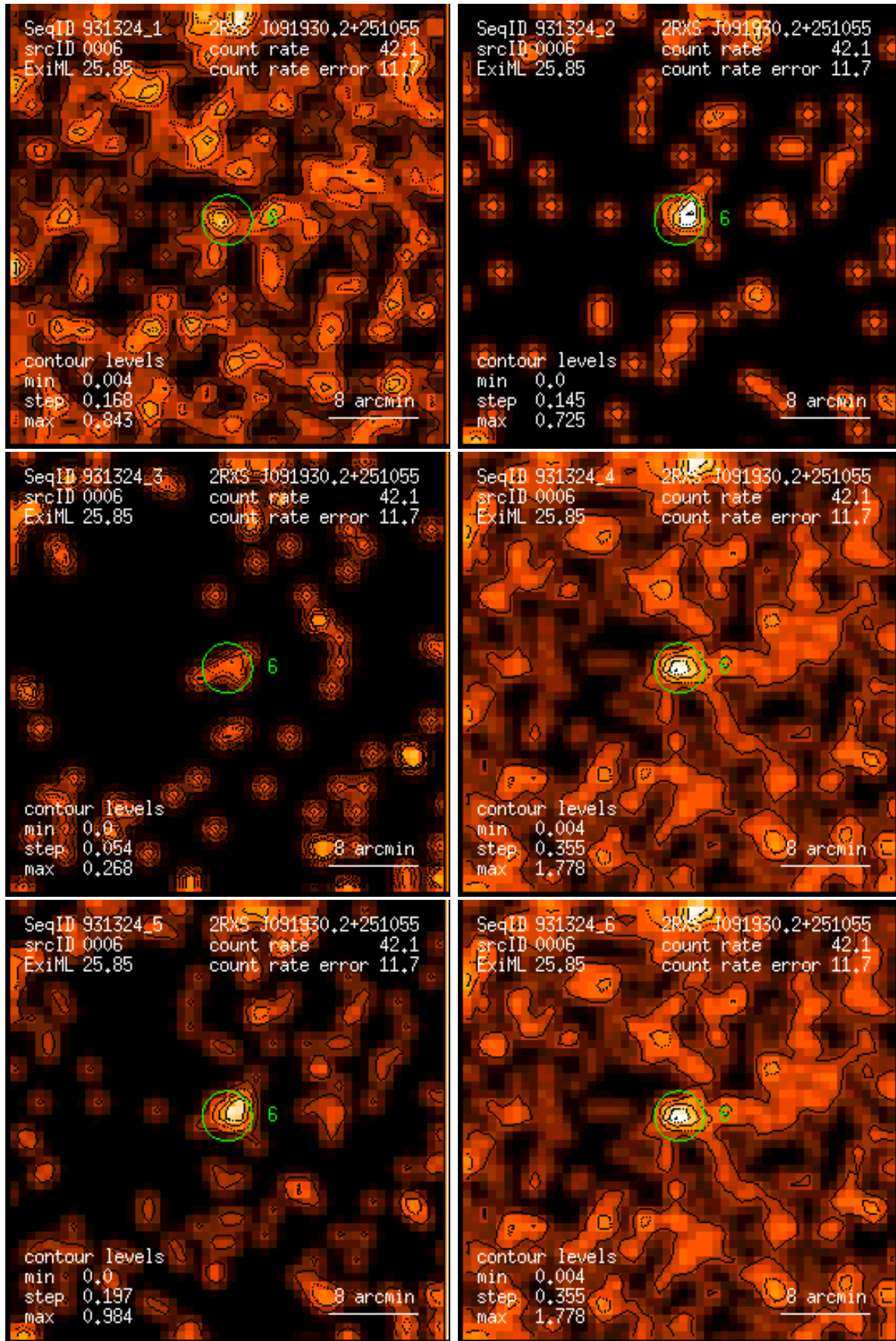
Figure 6: RASS 931324: detection 0006: band rate images, Gaussian filter: (1) PSPC channels 11 – 41, (2) 52 – 90, (3) 91 – 201, (4) 11 – 235, (5) 52 – 201, (6) 11 – 201. Broad band rates in counts/ks. Band rate contour levels in counts/ks/arcmin 2 .
