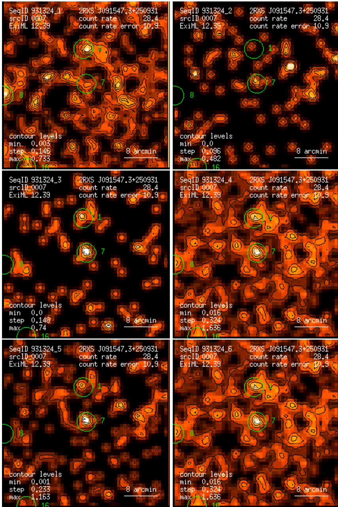
Figure 7: RASS 931324: detection 0007: band rate images, Gaussian filter: (1) PSPC channels 11 – 41, (2) 52 – 90, (3) 91 – 201, (4) 11 – 235, (5) 52 – 201, (6) 11 – 201. Broad band rates in counts/ks. Band rate contour levels in counts/ks/arcmin 2 .
