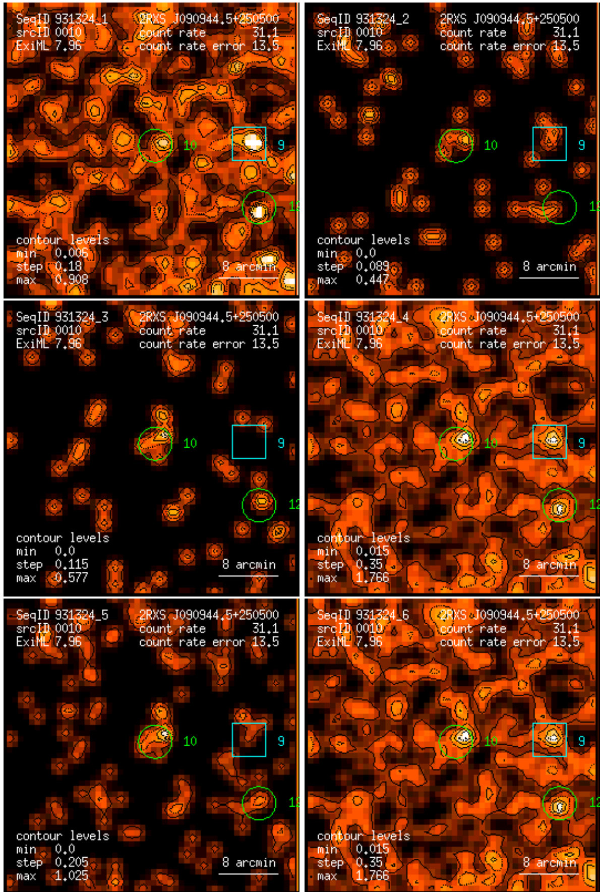
Figure 10: RASS 931324: detection 0010: band rate images, Gaussian filter: (1) PSPC channels 11 – 41, (2) 52 – 90, (3) 91 – 201, (4) 11 – 235, (5) 52 – 201, (6) 11 – 201. Broad band rates in counts/ks. Band rate contour levels in counts/ks/arcmin 2 .
