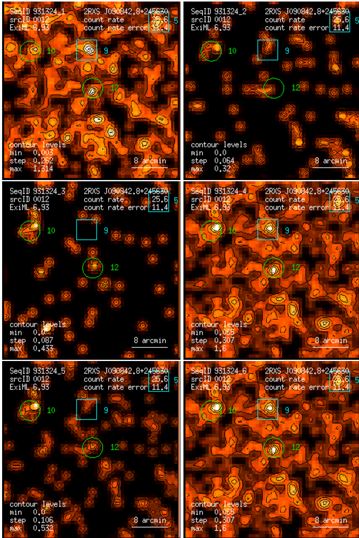
Figure 12: RASS 931324: detection 0012: band rate images, Gaussian filter: (1) PSPC channels 11 – 41, (2) 52 – 90, (3) 91 – 201, (4) 11 – 235, (5) 52 – 201, (6) 11 – 201. Broad band rates in counts/ks. Band rate contour levels in counts/ks/arcmin 2 .
