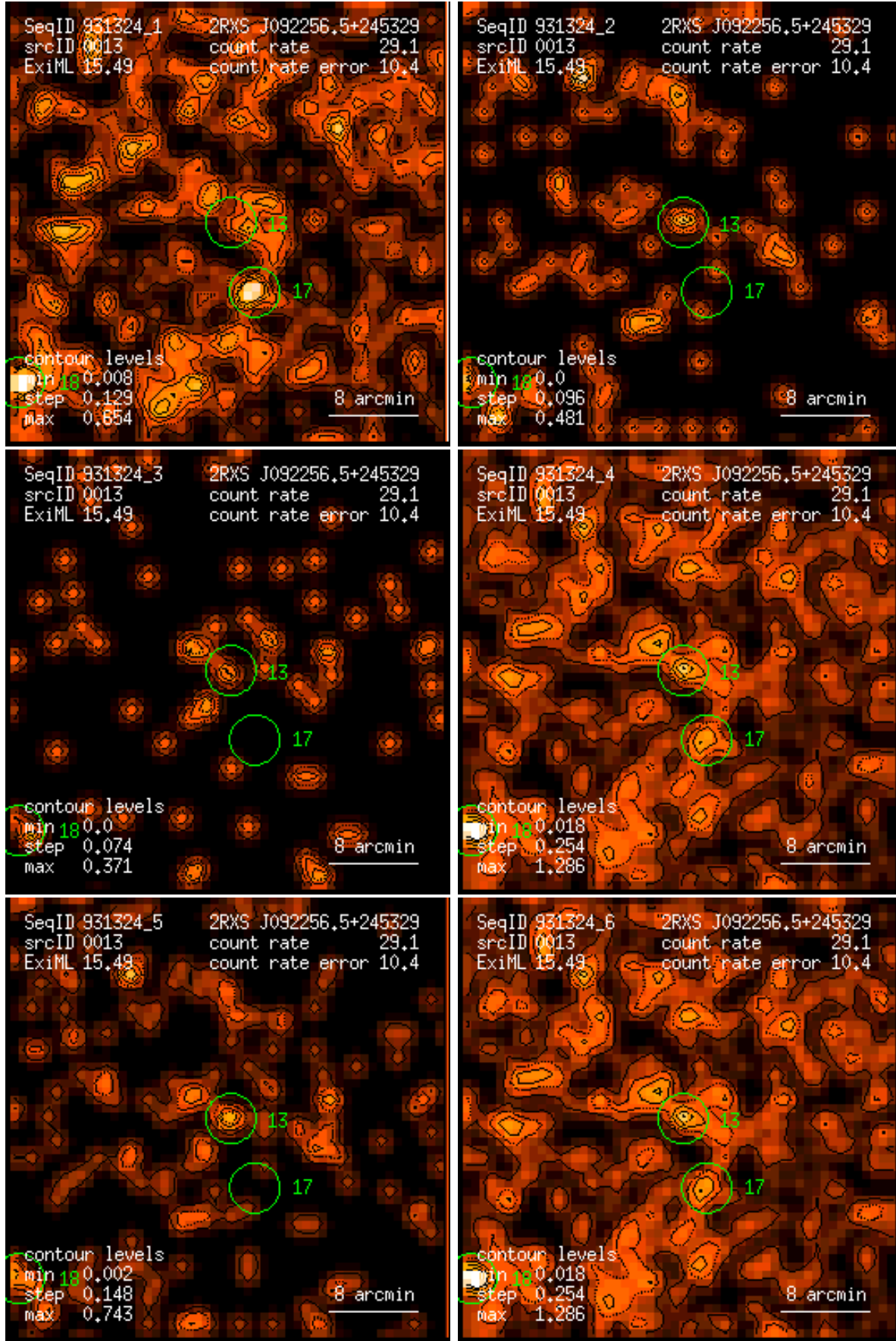
Figure 13: RASS 931324: detection 0013: band rate images, Gaussian filter: (1) PSPC channels 11 – 41, (2) 52 – 90, (3) 91 – 201, (4) 11 – 235, (5) 52 – 201, (6) 11 – 201. Broad band rates in counts/ks. Band rate contour levels in counts/ks/arcmin 2 .
