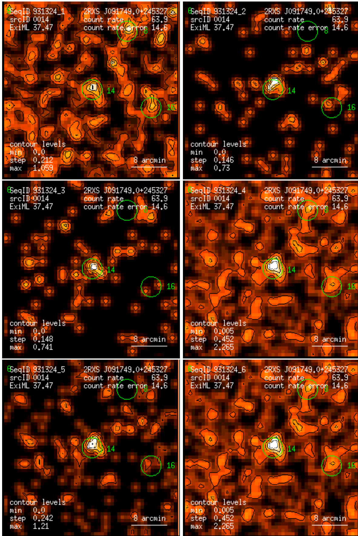
Figure 14: RASS 931324: detection 0014: band rate images, Gaussian filter: (1) PSPC channels 11 – 41, (2) 52 – 90, (3) 91 – 201, (4) 11 – 235, (5) 52 – 201, (6) 11 – 201. Broad band rates in counts/ks. Band rate contour levels in counts/ks/arcmin 2 .
