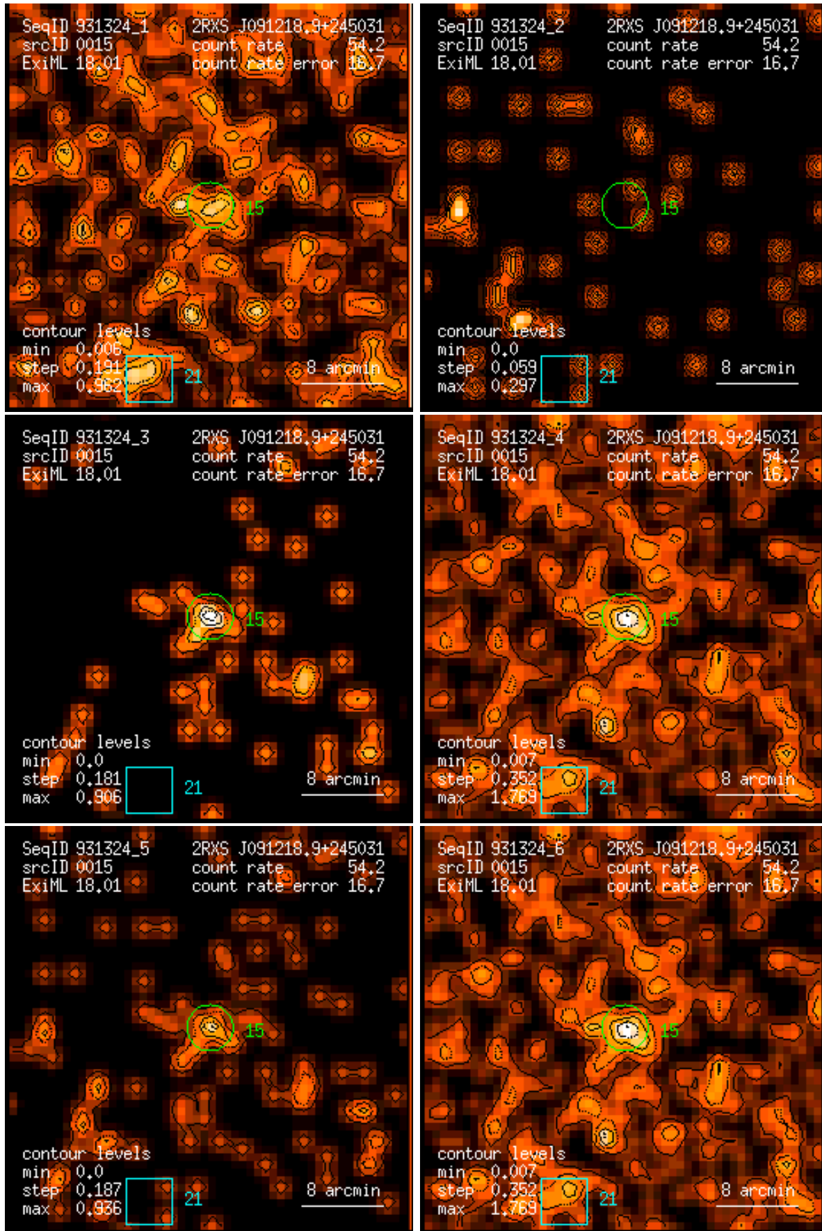
Figure 15: RASS 931324: detection 0015: band rate images, Gaussian filter: (1) PSPC channels 11 – 41, (2) 52 – 90, (3) 91 – 201, (4) 11 – 235, (5) 52 – 201, (6) 11 – 201. Broad band rates in counts/ks. Band rate contour levels in counts/ks/arcmin 2 .
