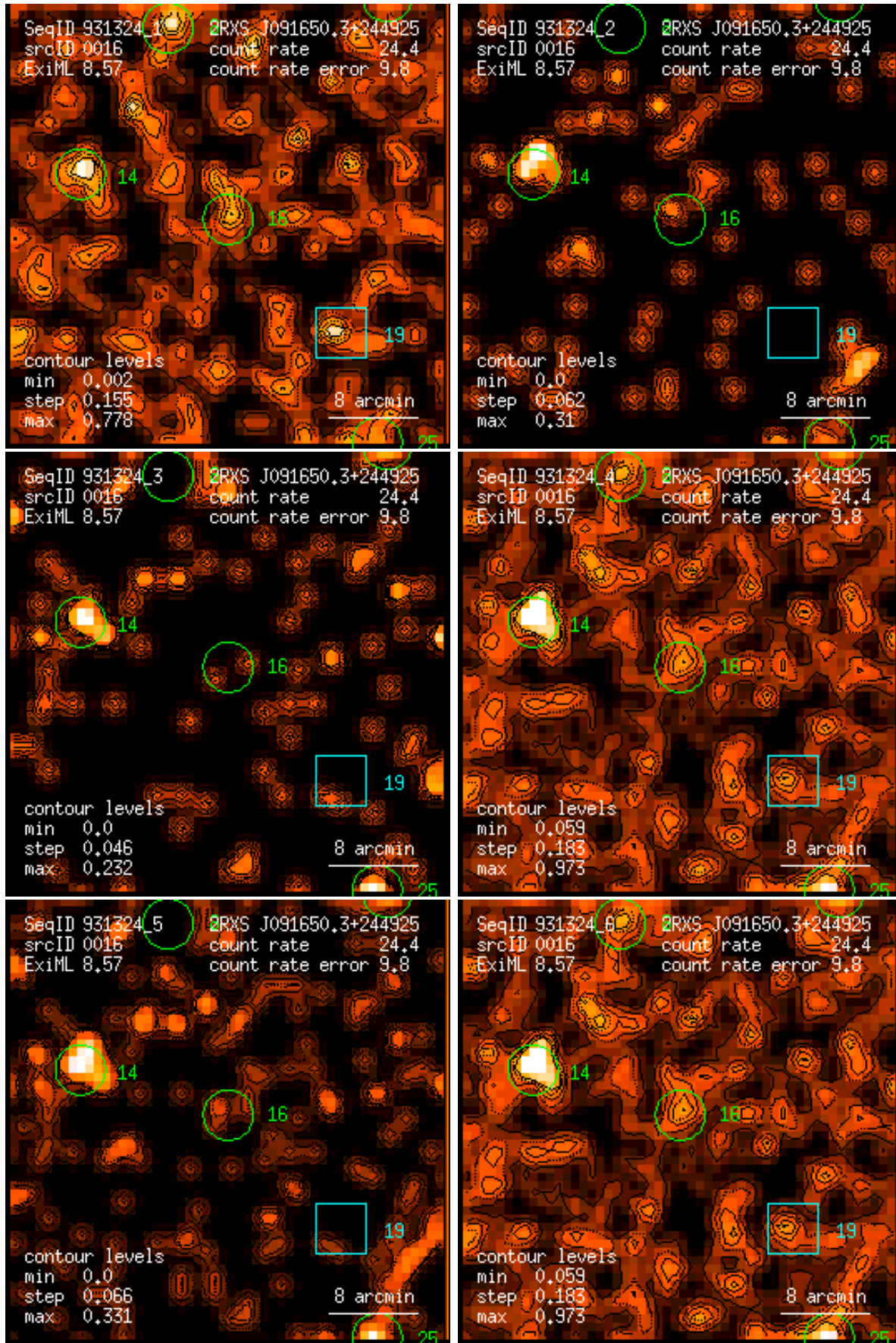
Figure 16: RASS 931324: detection 0016: band rate images, Gaussian filter: (1) PSPC channels 11 – 41, (2) 52 – 90, (3) 91 – 201, (4) 11 – 235, (5) 52 – 201, (6) 11 – 201. Broad band rates in counts/ks. Band rate contour levels in counts/ks/arcmin 2 .
