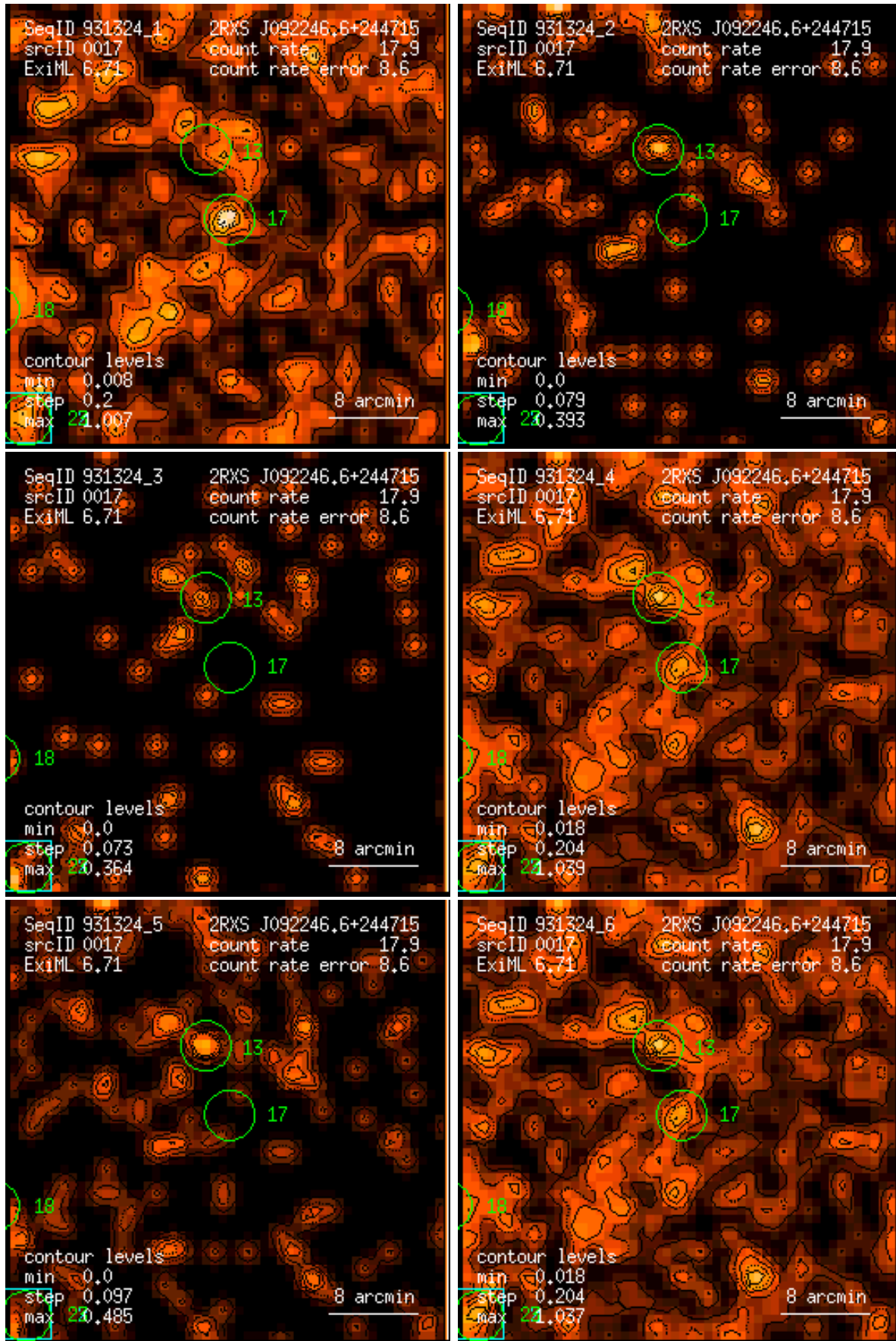
Figure 17: RASS 931324: detection 0017: band rate images, Gaussian filter: (1) PSPC channels 11 – 41, (2) 52 – 90, (3) 91 – 201, (4) 11 – 235, (5) 52 – 201, (6) 11 – 201. Broad band rates in counts/ks. Band rate contour levels in counts/ks/arcmin 2 .
