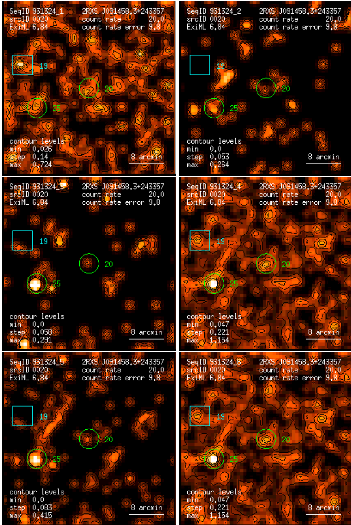
Figure 20: RASS 931324: detection 0020: band rate images, Gaussian filter: (1) PSPC channels 11 – 41, (2) 52 – 90, (3) 91 – 201, (4) 11 – 235, (5) 52 – 201, (6) 11 – 201. Broad band rates in counts/ks. Band rate contour levels in counts/ks/arcmin 2 .
