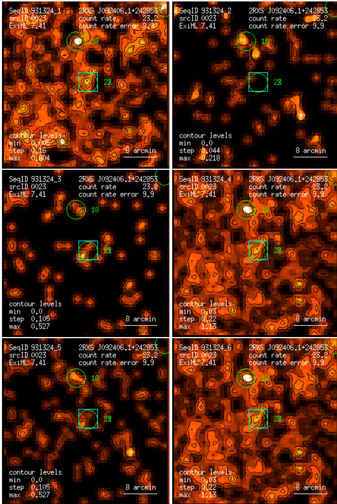
Figure 23: RASS 931324: detection 0023: band rate images, Gaussian filter: (1) PSPC channels 11 – 41, (2) 52 – 90, (3) 91 – 201, (4) 11 – 235, (5) 52 – 201, (6) 11 – 201. Broad band rates in counts/ks. Band rate contour levels in counts/ks/arcmin 2 .
