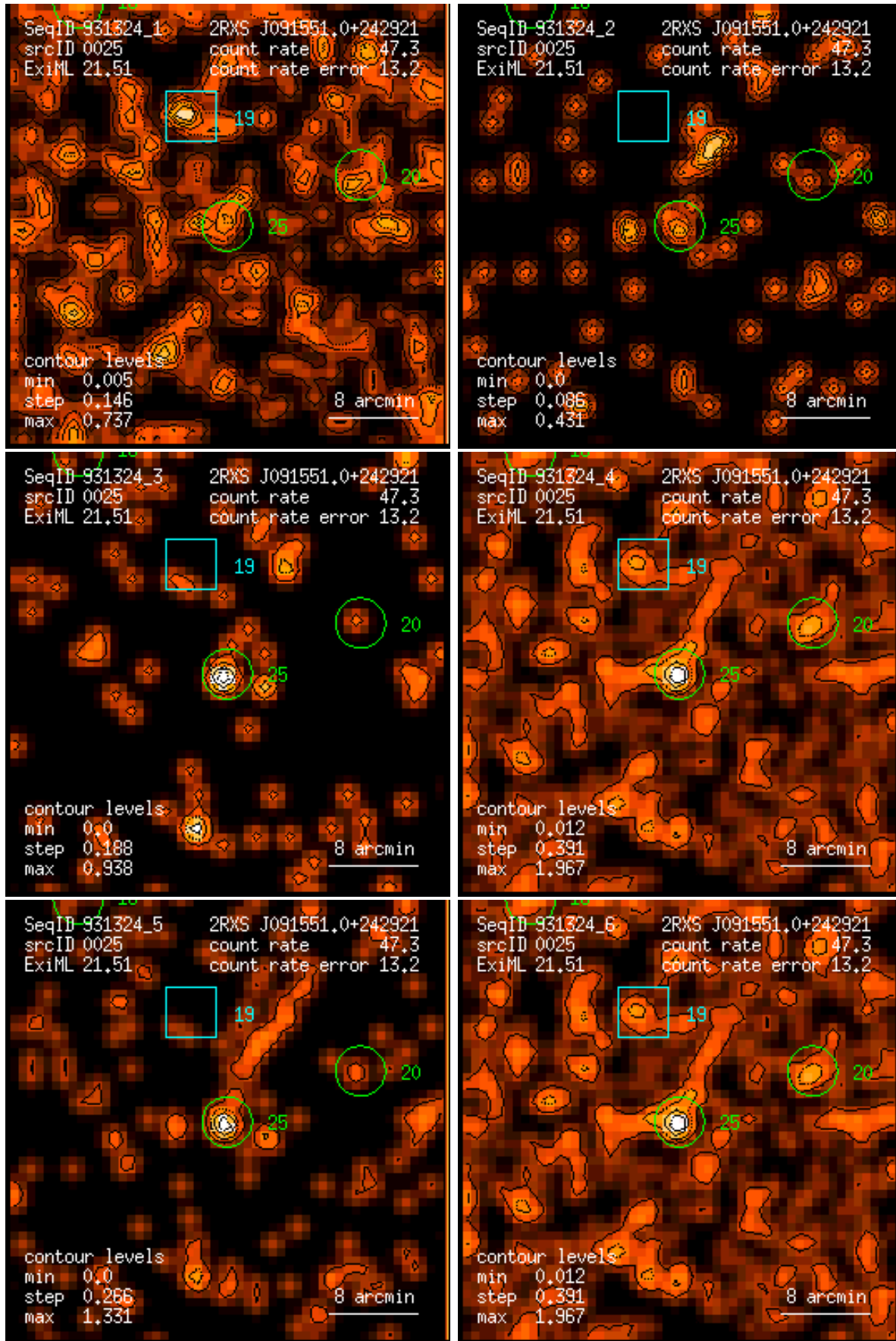
Figure 25: RASS 931324: detection 0025: band rate images, Gaussian filter: (1) PSPC channels 11 – 41, (2) 52 – 90, (3) 91 – 201, (4) 11 – 235, (5) 52 – 201, (6) 11 – 201. Broad band rates in counts/ks. Band rate contour levels in counts/ks/arcmin 2 .
