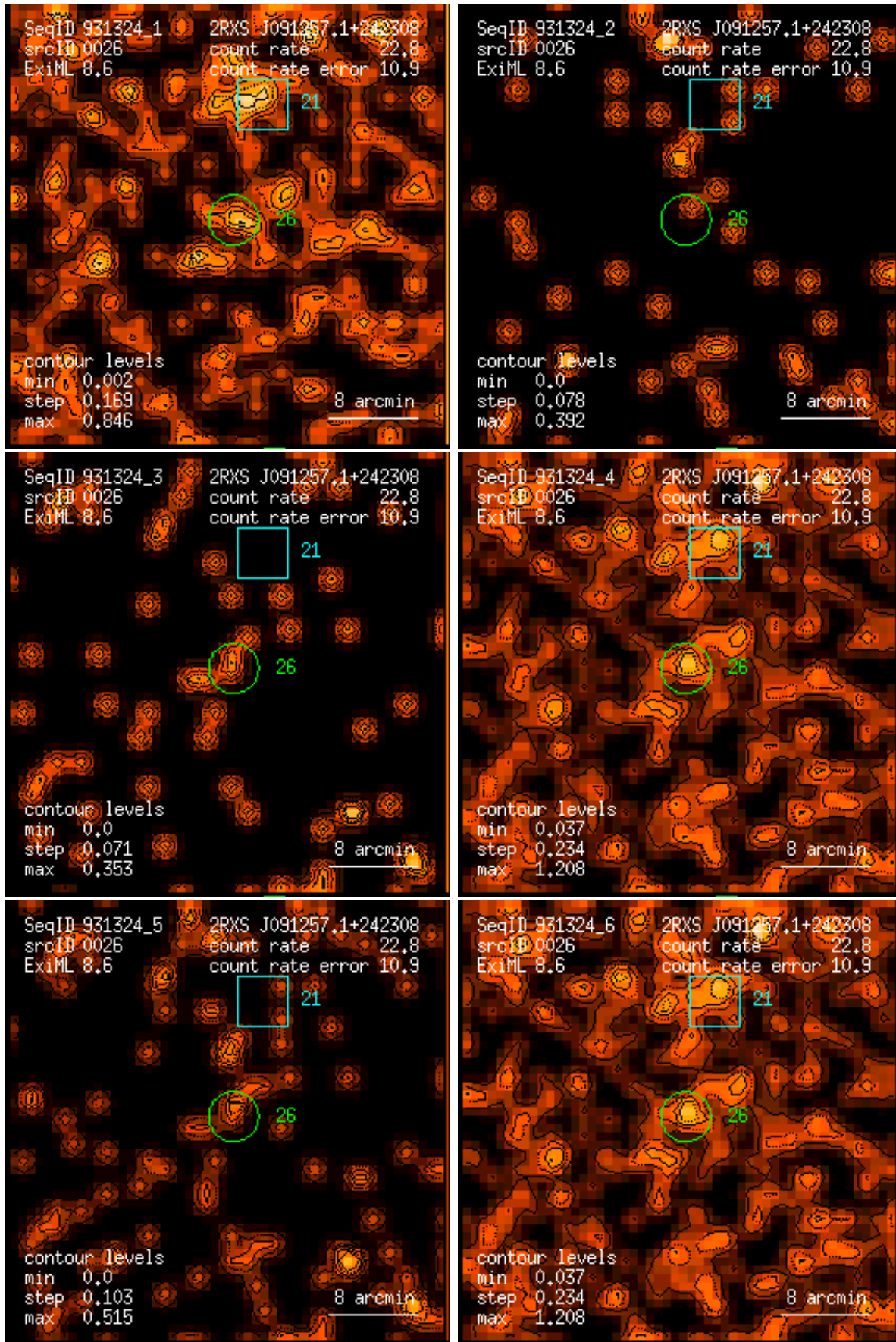
Figure 26: RASS 931324: detection 0026: band rate images, Gaussian filter: (1) PSPC channels 11 – 41, (2) 52 – 90, (3) 91 – 201, (4) 11 – 235, (5) 52 – 201, (6) 11 – 201. Broad band rates in counts/ks. Band rate contour levels in counts/ks/arcmin 2 .
