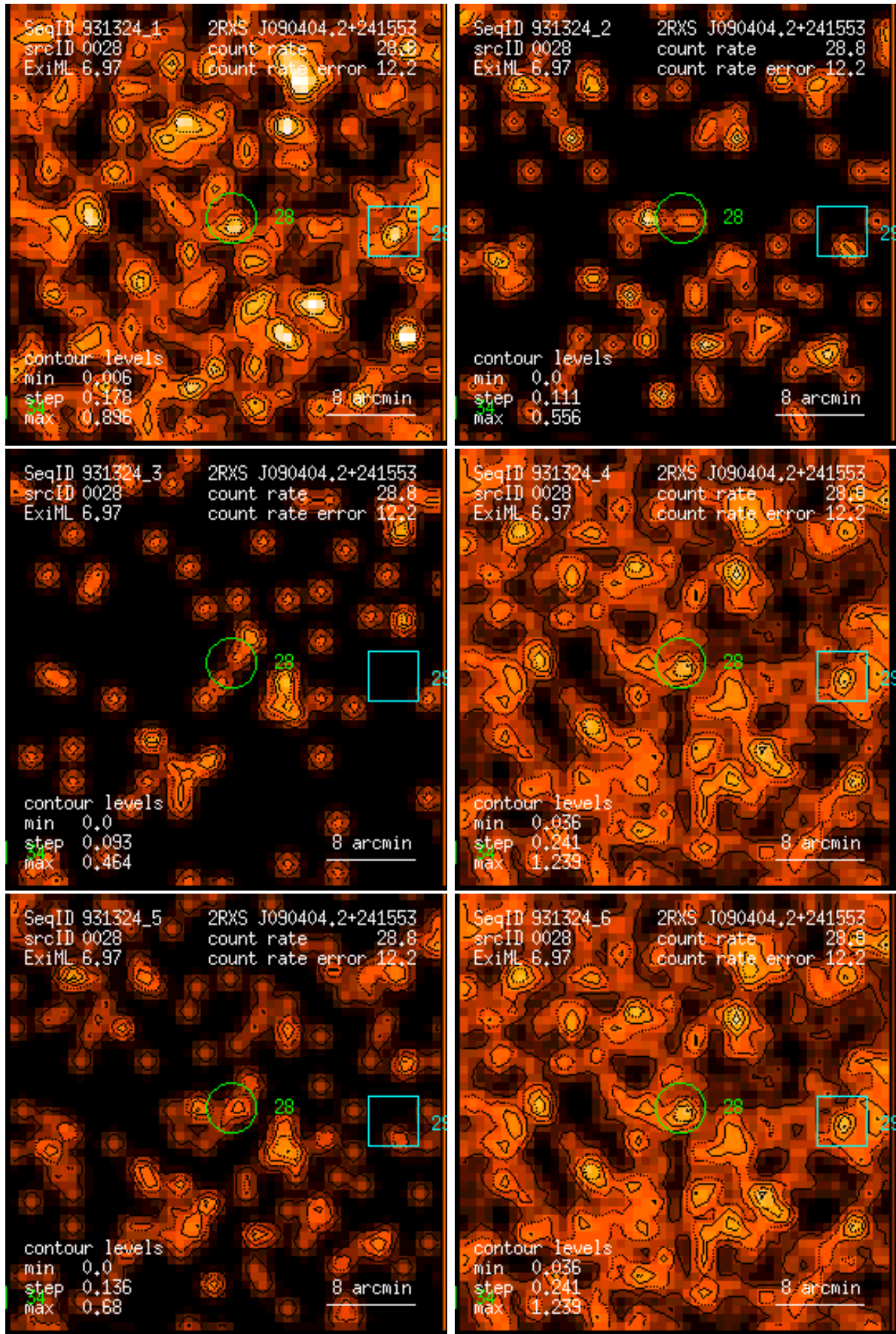
Figure 28: RASS 931324: detection 0028: band rate images, Gaussian filter: (1) PSPC channels 11 – 41, (2) 52 – 90, (3) 91 – 201, (4) 11 – 235, (5) 52 – 201, (6) 11 – 201. Broad band rates in counts/ks. Band rate contour levels in counts/ks/arcmin 2 .
