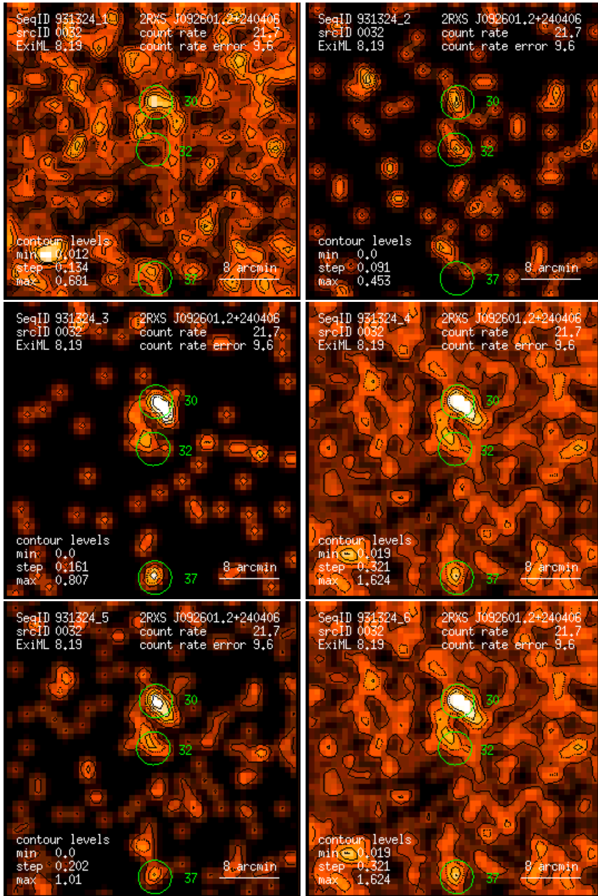
Figure 32: RASS 931324: detection 0032: band rate images, Gaussian filter: (1) PSPC channels 11 – 41, (2) 52 – 90, (3) 91 – 201, (4) 11 – 235, (5) 52 – 201, (6) 11 – 201. Broad band rates in counts/ks. Band rate contour levels in counts/ks/arcmin 2 .
