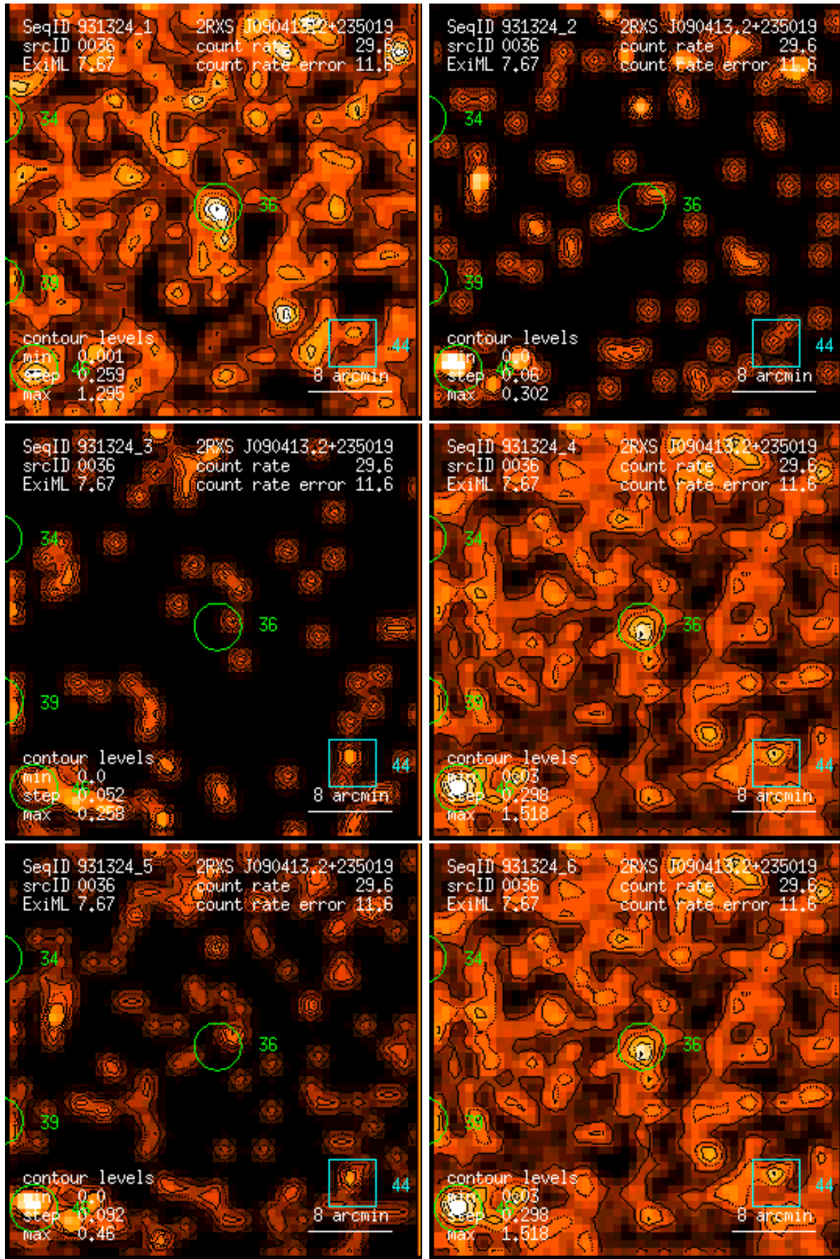
Figure 36: RASS 931324: detection 0036: band rate images, Gaussian filter: (1) PSPC channels 11 – 41, (2) 52 – 90, (3) 91 – 201, (4) 11 – 235, (5) 52 – 201, (6) 11 – 201. Broad band rates in counts/ks. Band rate contour levels in counts/ks/arcmin 2 .
