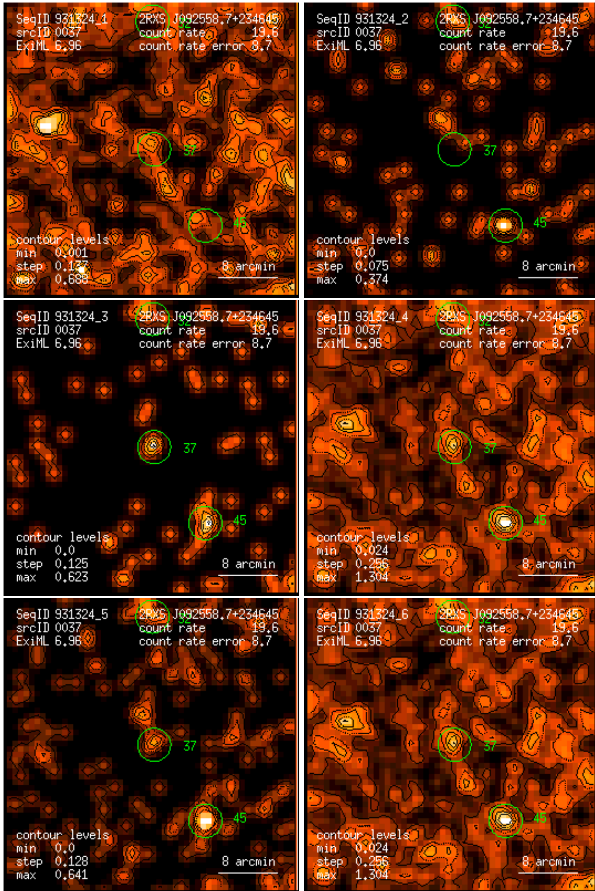
Figure 37: RASS 931324: detection 0037: band rate images, Gaussian filter: (1) PSPC channels 11 – 41, (2) 52 – 90, (3) 91 – 201, (4) 11 – 235, (5) 52 – 201, (6) 11 – 201. Broad band rates in counts/ks. Band rate contour levels in counts/ks/arcmin 2 .
