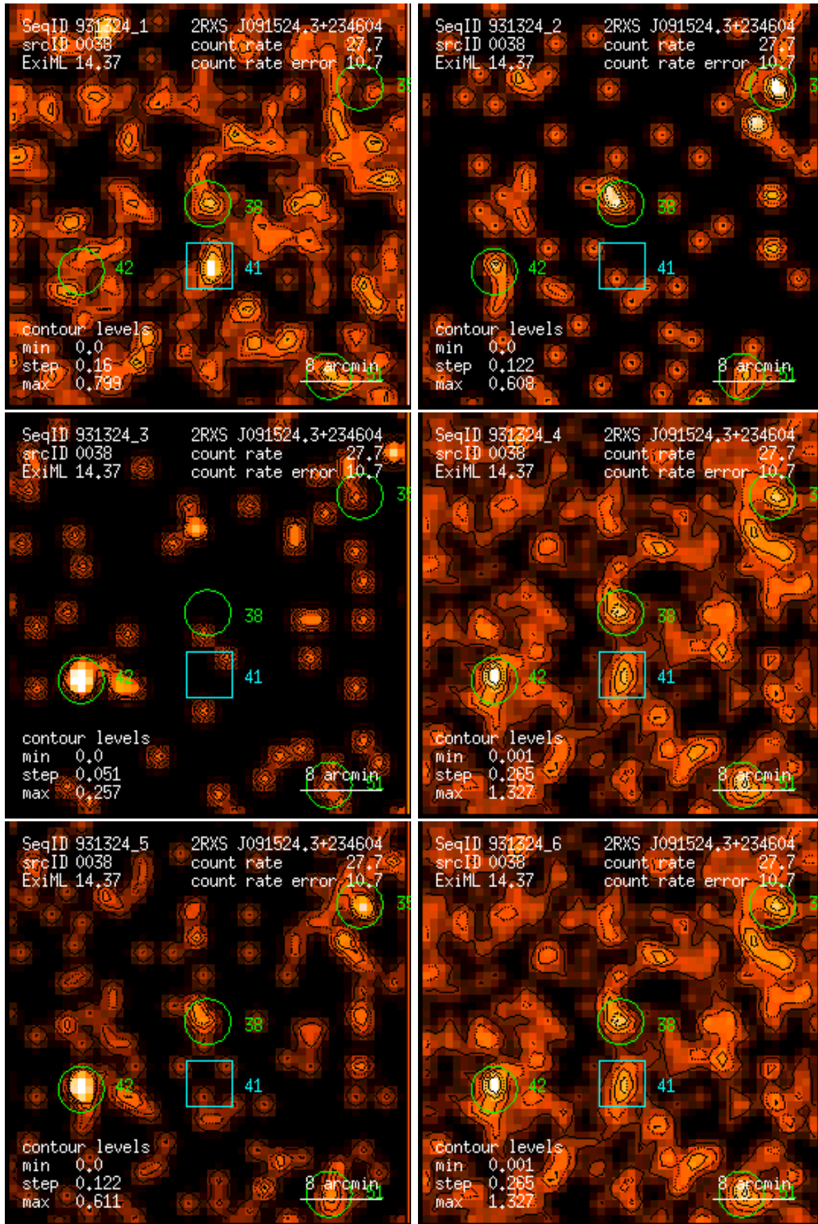
Figure 38: RASS 931324: detection 0038: band rate images, Gaussian filter: (1) PSPC channels 11 – 41, (2) 52 – 90, (3) 91 – 201, (4) 11 – 235, (5) 52 – 201, (6) 11 – 201. Broad band rates in counts/ks. Band rate contour levels in counts/ks/arcmin 2 .
