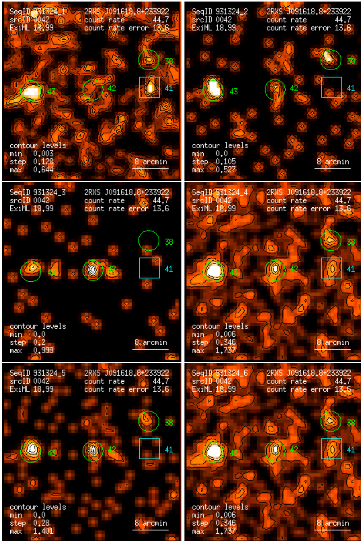
Figure 42: RASS 931324: detection 0042: band rate images, Gaussian filter: (1) PSPC channels 11 – 41, (2) 52 – 90, (3) 91 – 201, (4) 11 – 235, (5) 52 – 201, (6) 11 – 201. Broad band rates in counts/ks. Band rate contour levels in counts/ks/arcmin 2 .
