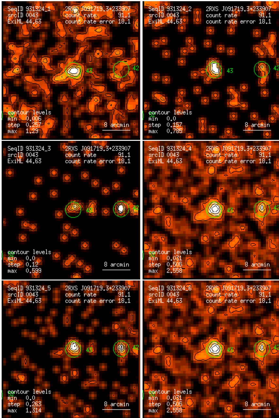
Figure 43: RASS 931324: detection 0043: band rate images, Gaussian filter: (1) PSPC channels 11 – 41, (2) 52 – 90, (3) 91 – 201, (4) 11 – 235, (5) 52 – 201, (6) 11 – 201. Broad band rates in counts/ks. Band rate contour levels in counts/ks/arcmin 2 .
