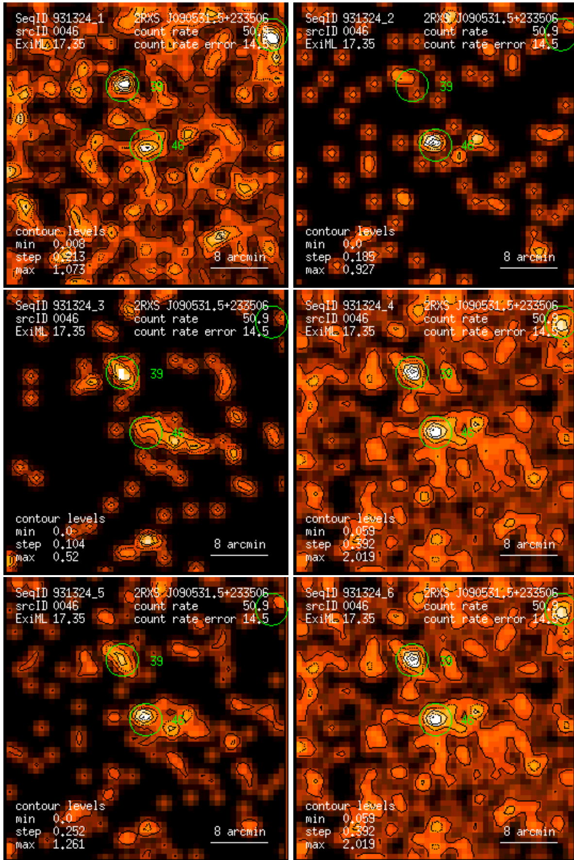
Figure 46: RASS 931324: detection 0046: band rate images, Gaussian filter: (1) PSPC channels 11 – 41, (2) 52 – 90, (3) 91 – 201, (4) 11 – 235, (5) 52 – 201, (6) 11 – 201. Broad band rates in counts/ks. Band rate contour levels in counts/ks/arcmin 2 .
