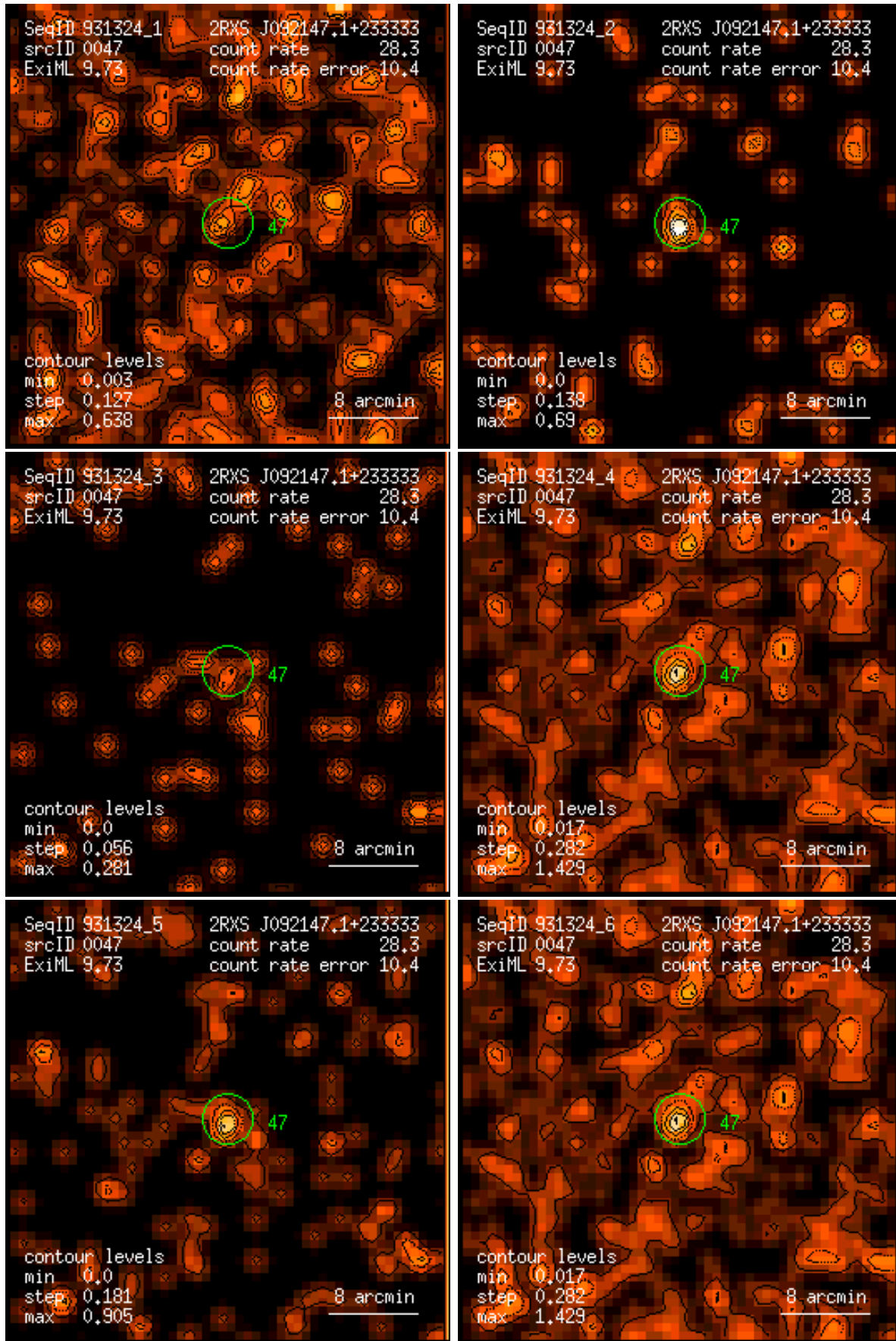
Figure 47: RASS 931324: detection 0047: band rate images, Gaussian filter: (1) PSPC channels 11 – 41, (2) 52 – 90, (3) 91 – 201, (4) 11 – 235, (5) 52 – 201, (6) 11 – 201. Broad band rates in counts/ks. Band rate contour levels in counts/ks/arcmin 2 .
