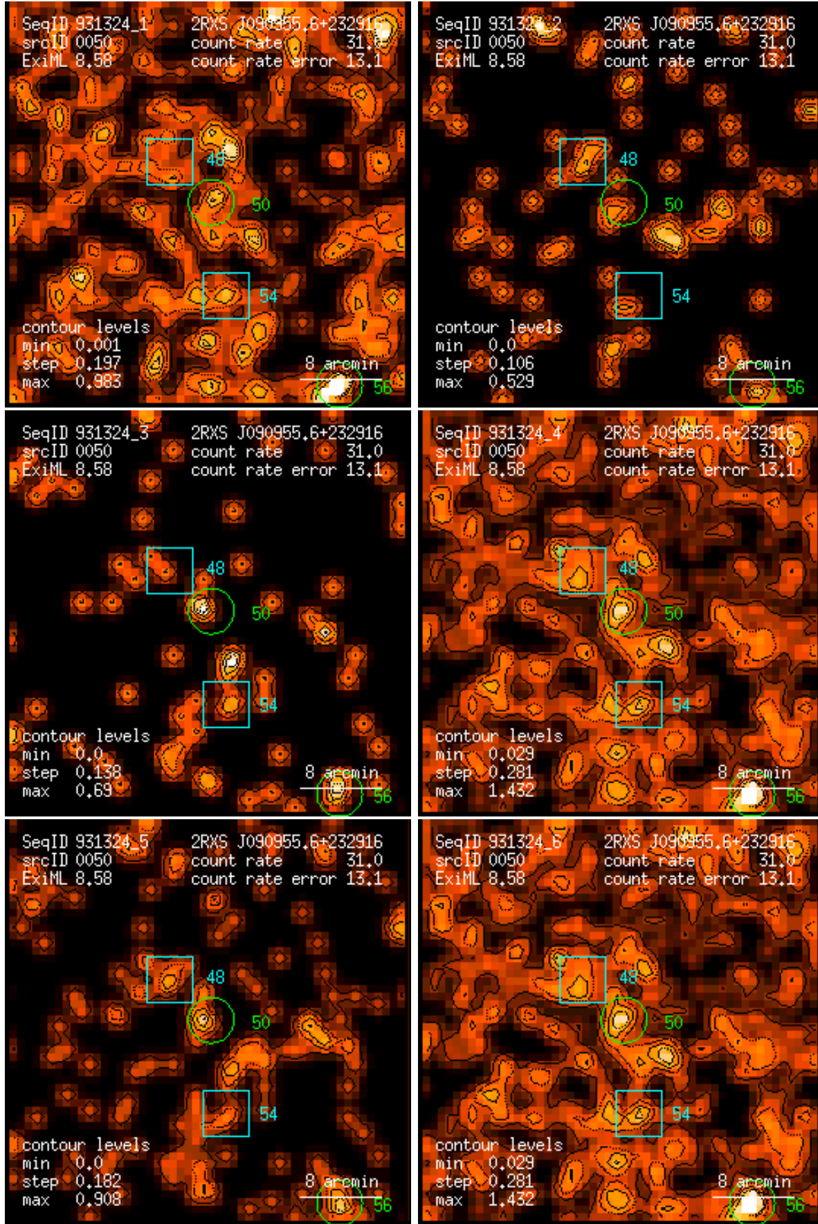
Figure 50: RASS 931324: detection 0050: band rate images, Gaussian filter: (1) PSPC channels 11 – 41, (2) 52 – 90, (3) 91 – 201, (4) 11 – 235, (5) 52 – 201, (6) 11 – 201. Broad band rates in counts/ks. Band rate contour levels in counts/ks/arcmin 2 .
