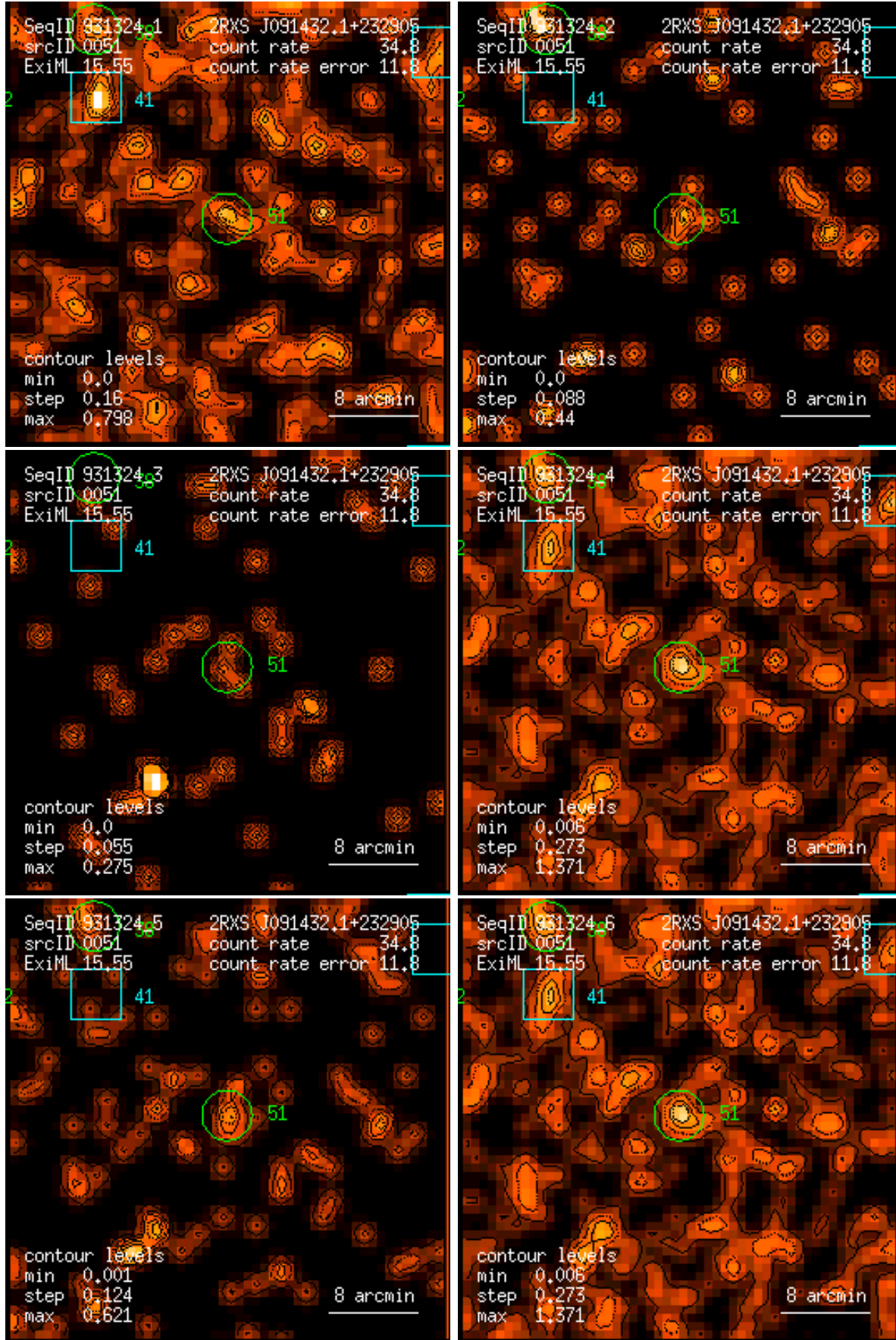
Figure 51: RASS 931324: detection 0051: band rate images, Gaussian filter: (1) PSPC channels 11 – 41, (2) 52 – 90, (3) 91 – 201, (4) 11 – 235, (5) 52 – 201, (6) 11 – 201. Broad band rates in counts/ks. Band rate contour levels in counts/ks/arcmin 2 .
