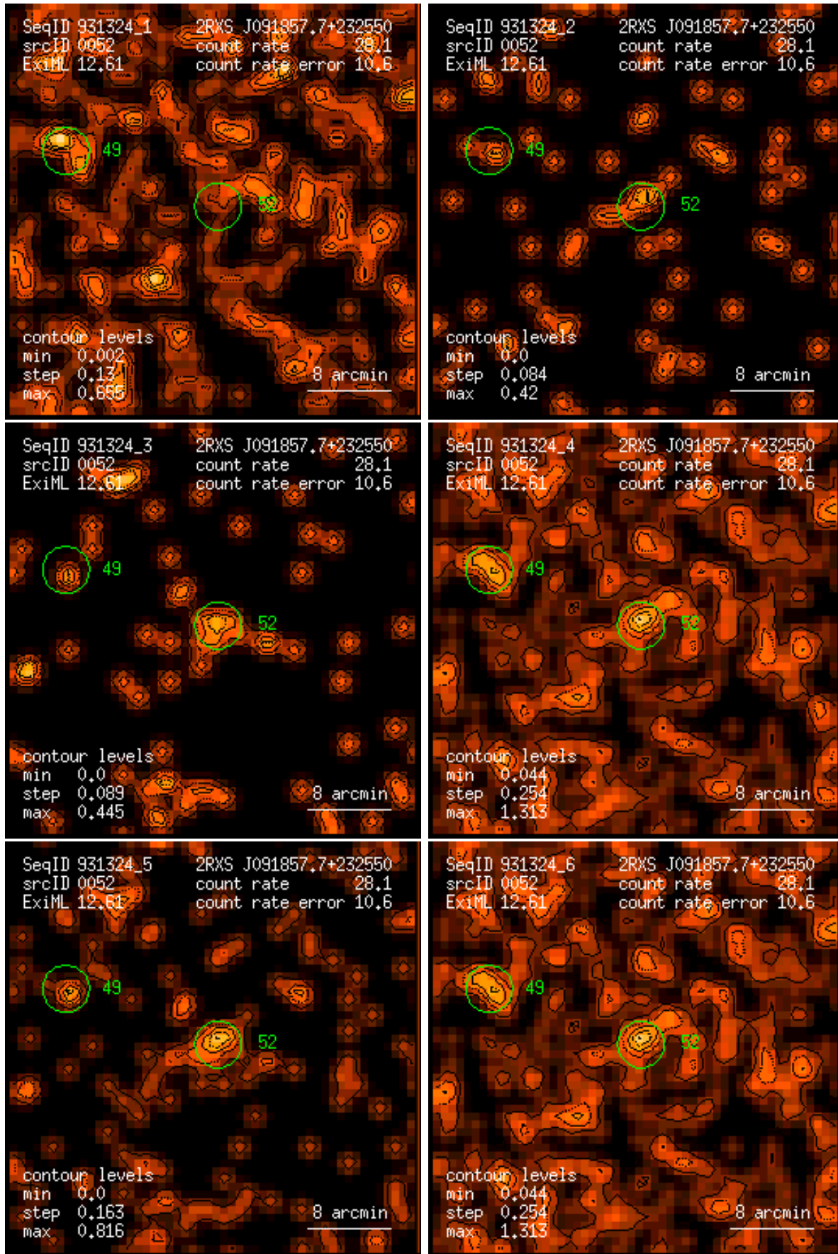
Figure 52: RASS 931324: detection 0052: band rate images, Gaussian filter: (1) PSPC channels 11 – 41, (2) 52 – 90, (3) 91 – 201, (4) 11 – 235, (5) 52 – 201, (6) 11 – 201. Broad band rates in counts/ks. Band rate contour levels in counts/ks/arcmin 2 .
