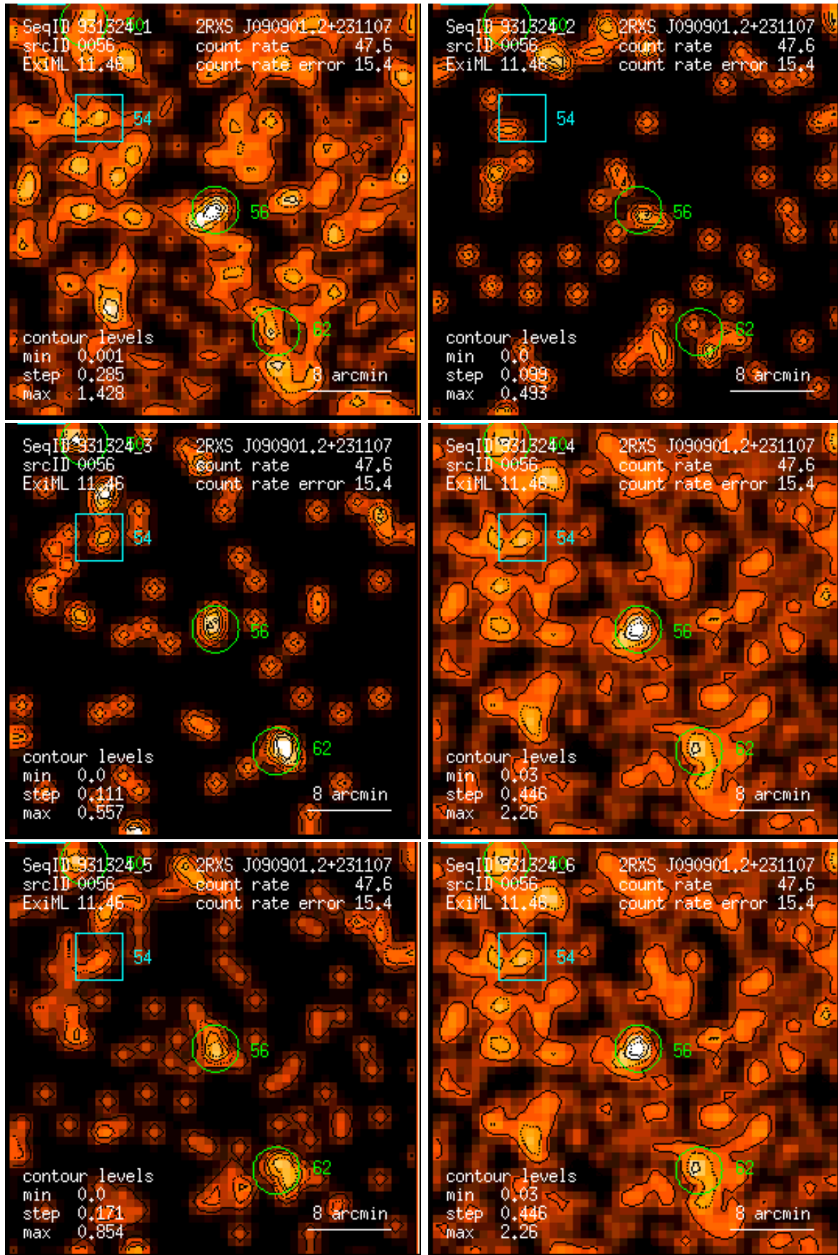
Figure 56: RASS 931324: detection 0056: band rate images, Gaussian filter: (1) PSPC channels 11 – 41, (2) 52 – 90, (3) 91 – 201, (4) 11 – 235, (5) 52 – 201, (6) 11 – 201. Broad band rates in counts/ks. Band rate contour levels in counts/ks/arcmin 2 .
