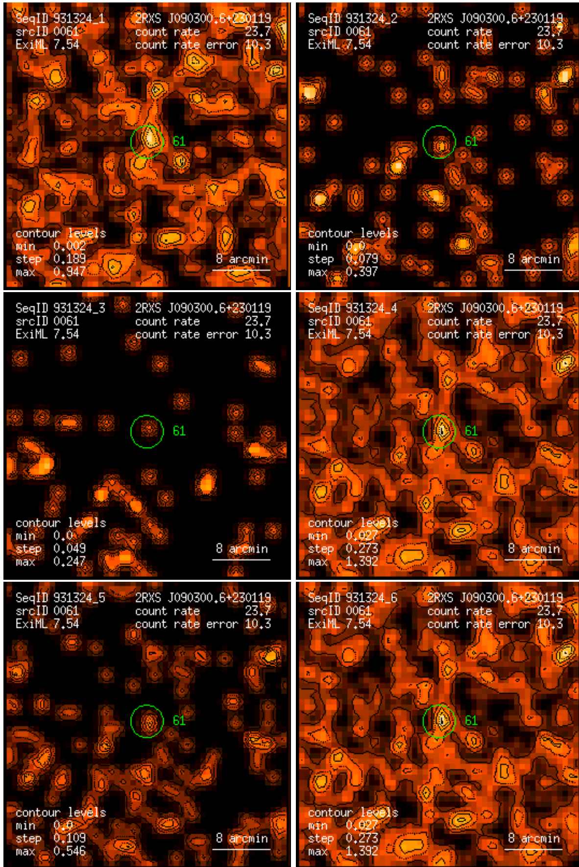
Figure 61: RASS 931324: detection 0061: band rate images, Gaussian filter: (1) PSPC channels 11 – 41, (2) 52 – 90, (3) 91 – 201, (4) 11 – 235, (5) 52 – 201, (6) 11 – 201. Broad band rates in counts/ks. Band rate contour levels in counts/ks/arcmin 2 .
