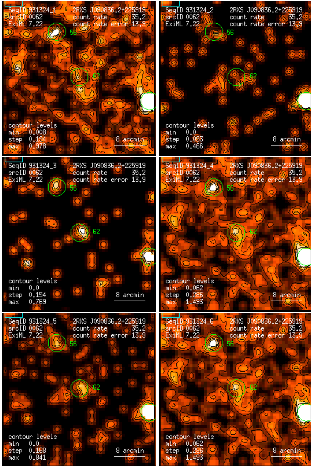
Figure 62: RASS 931324: detection 0062: band rate images, Gaussian filter: (1) PSPC channels 11 – 41, (2) 52 – 90, (3) 91 – 201, (4) 11 – 235, (5) 52 – 201, (6) 11 – 201. Broad band rates in counts/ks. Band rate contour levels in counts/ks/arcmin 2 .
