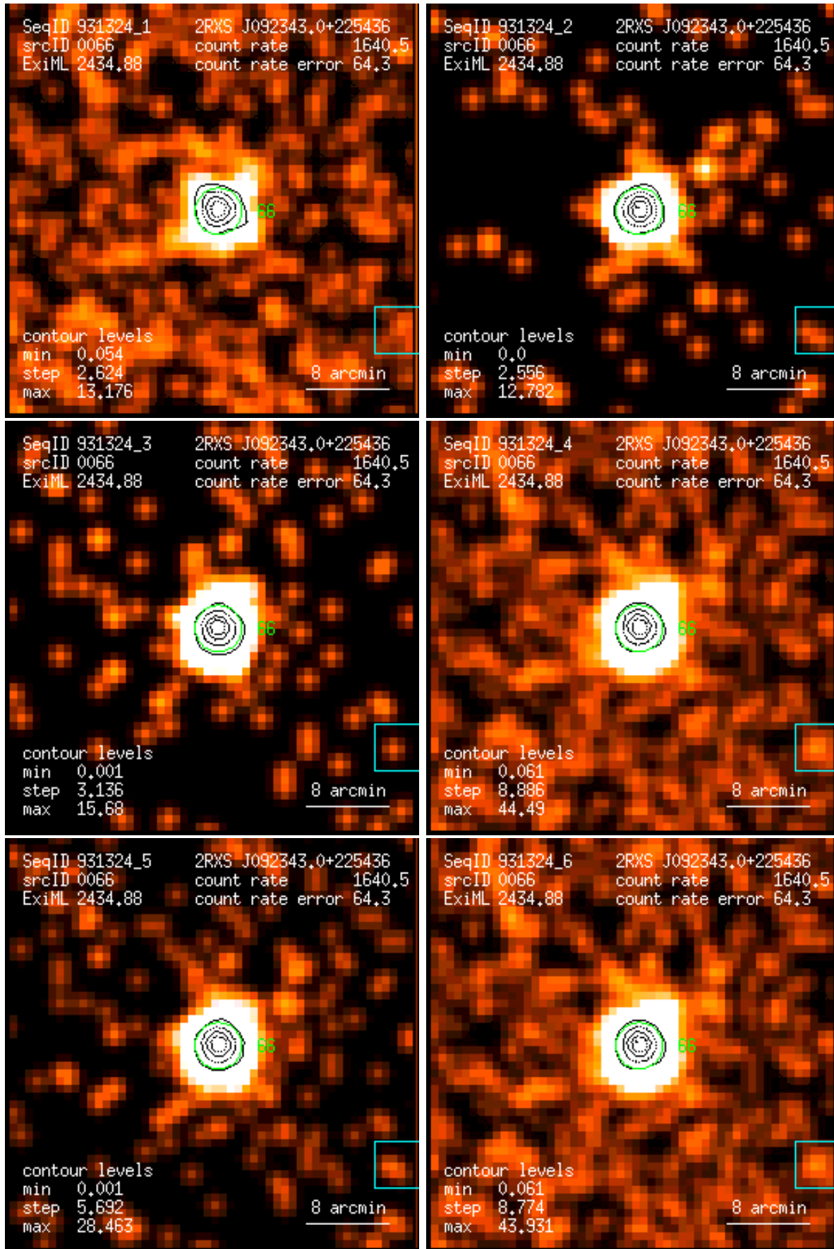
Figure 66: RASS 931324: detection 0066: band rate images, Gaussian filter: (1) PSPC channels 11 – 41, (2) 52 – 90, (3) 91 – 201, (4) 11 – 235, (5) 52 – 201, (6) 11 – 201. Broad band rates in counts/ks. Band rate contour levels in counts/ks/arcmin 2 .
