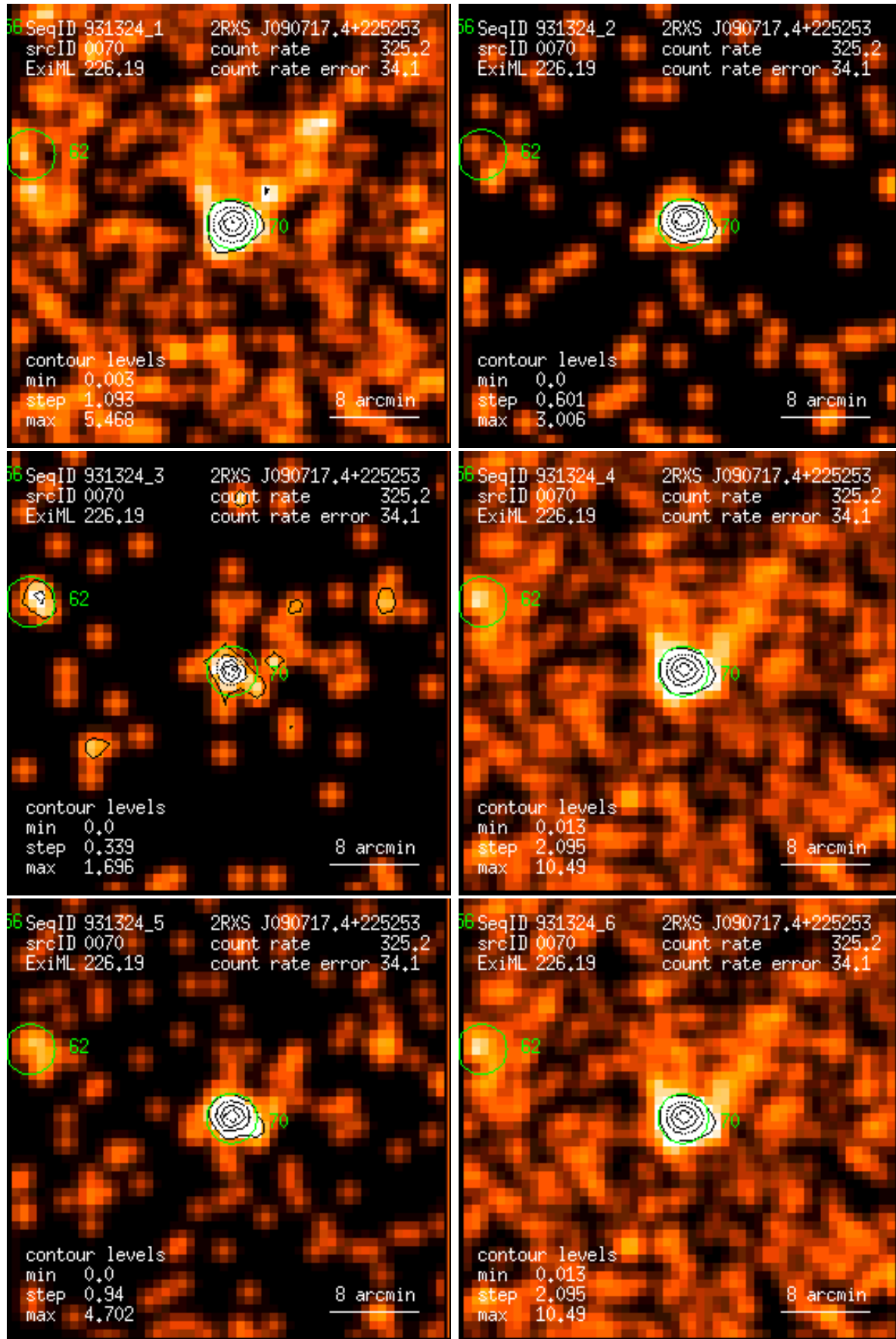
Figure 70: RASS 931324: detection 0070: band rate images, Gaussian filter: (1) PSPC channels 11 – 41, (2) 52 – 90, (3) 91 – 201, (4) 11 – 235, (5) 52 – 201, (6) 11 – 201. Broad band rates in counts/ks. Band rate contour levels in counts/ks/arcmin 2 .
